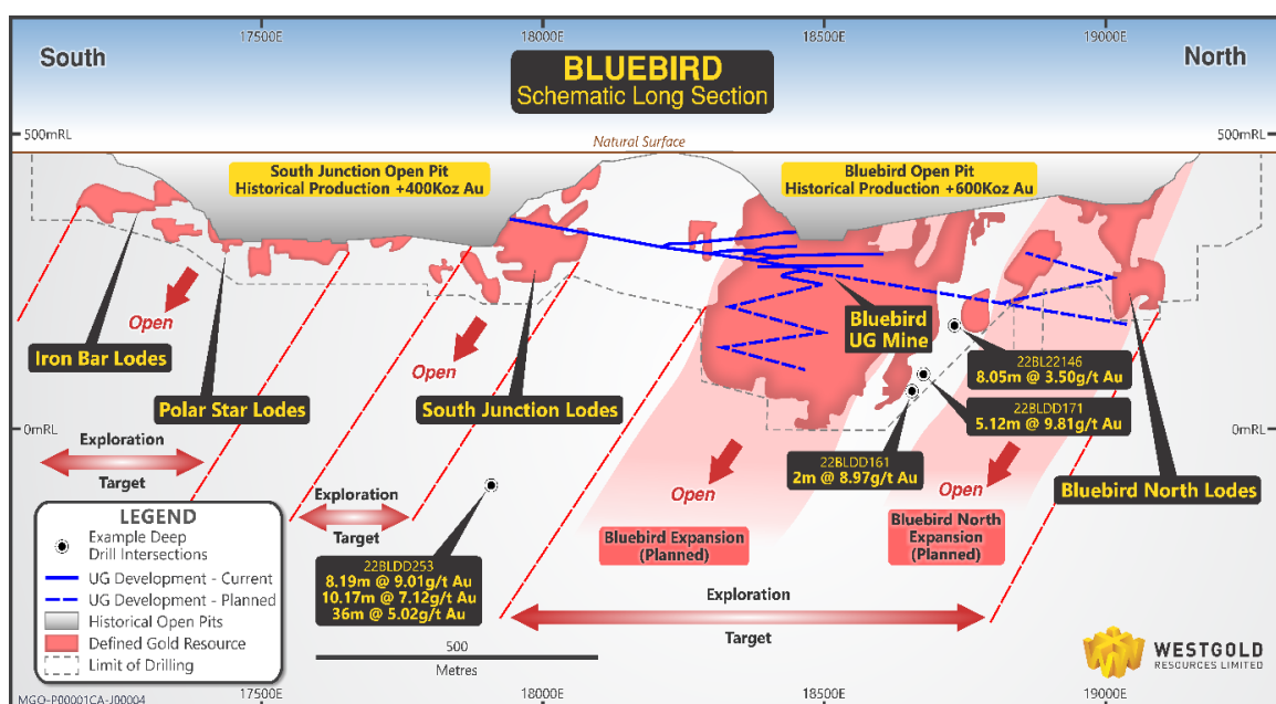
Figure 1: Bluebird Schematic Long-Section
