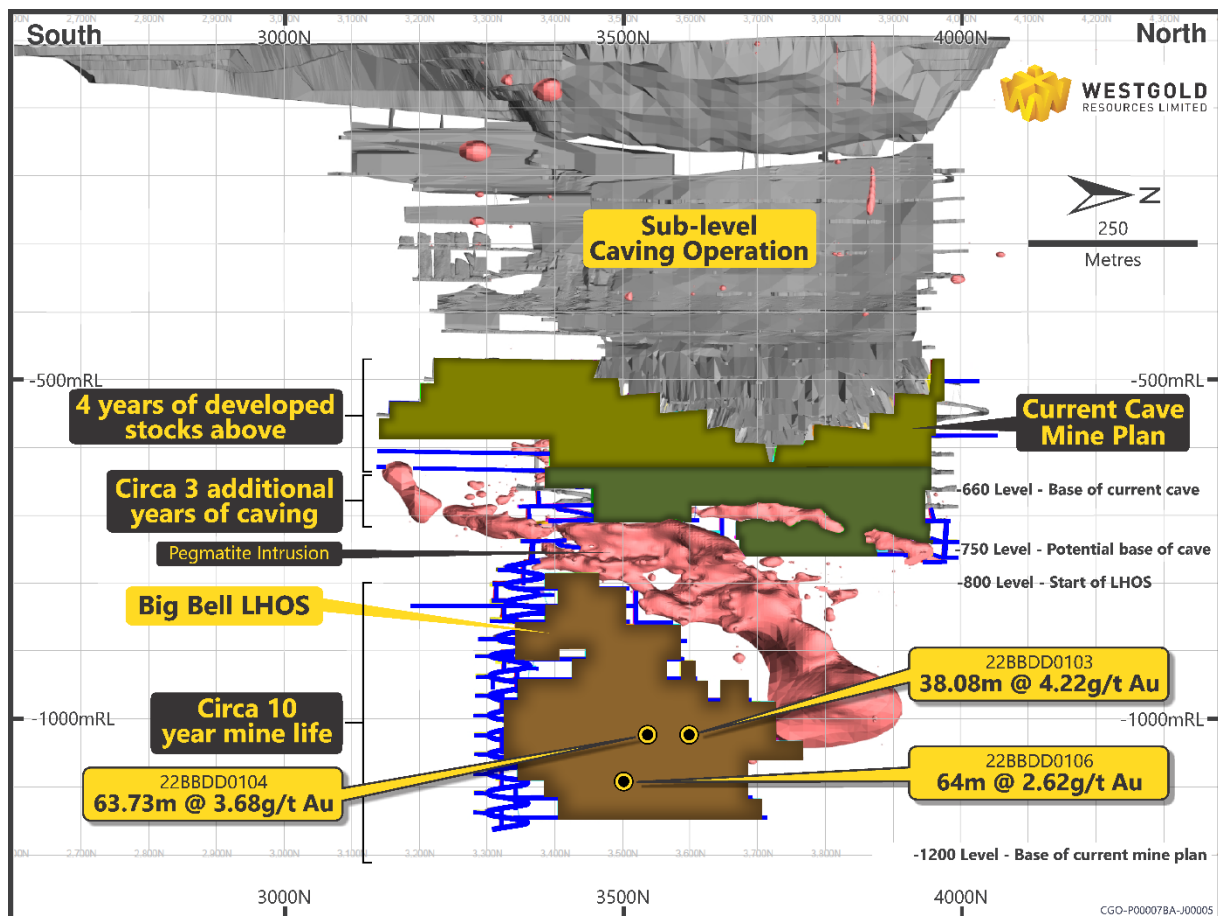
Figure 1: Proposed Big Bell Expansion mine layout with recent drill results in Expansion Plan area
