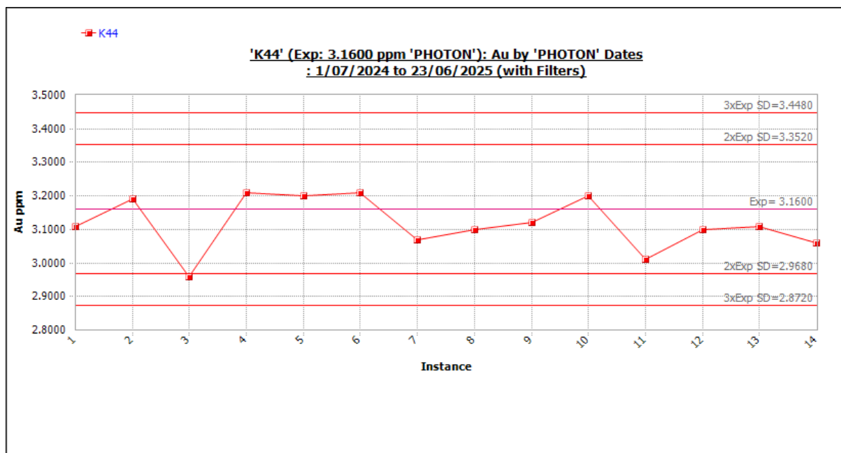
Figure 11-66 Standard K44 outliers included. Source: Westgold.
