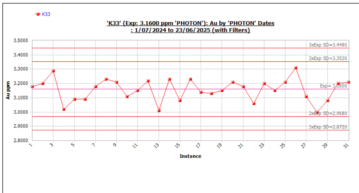
Figure 11-54 Standard K33 outliers included. Source: Westgold.
