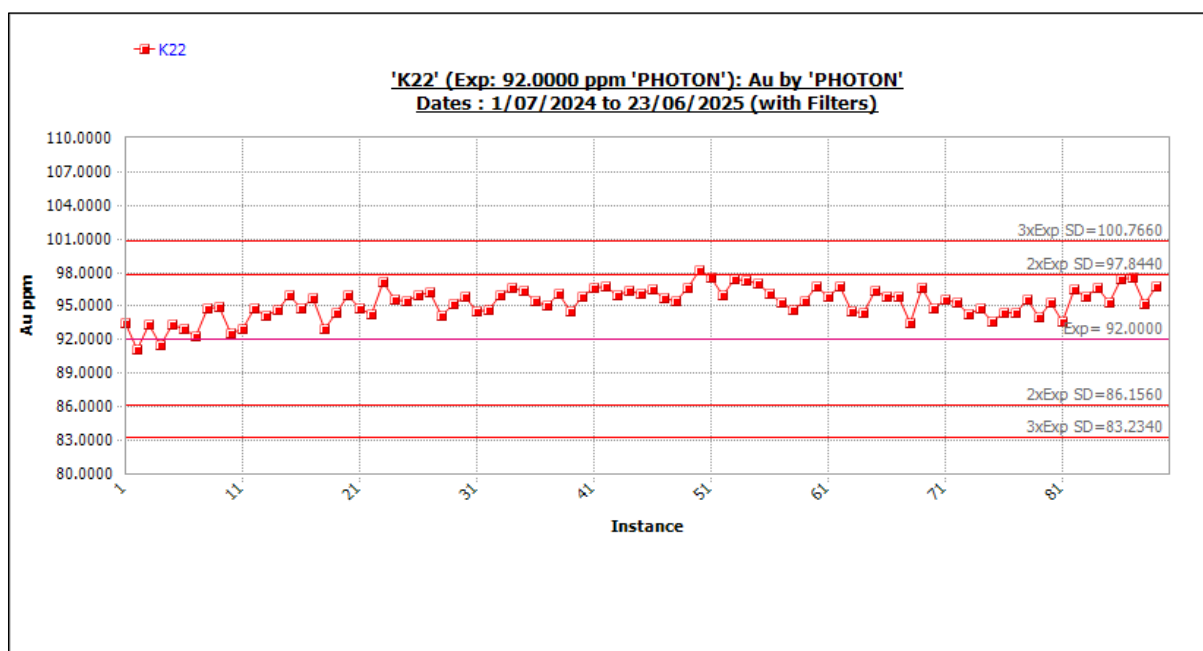
Figure 11-35 Standard K22 outliers included. Source: Westgold.
