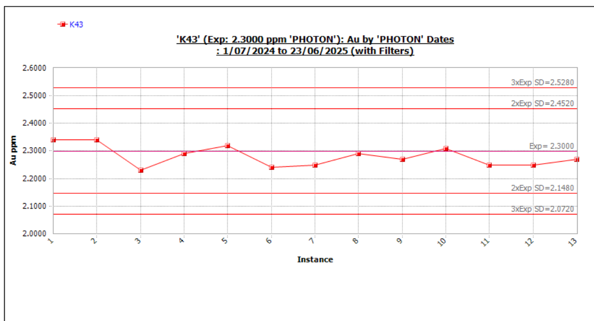
Figure 11-65 Standard K43 outliers included. Source: Westgold.
