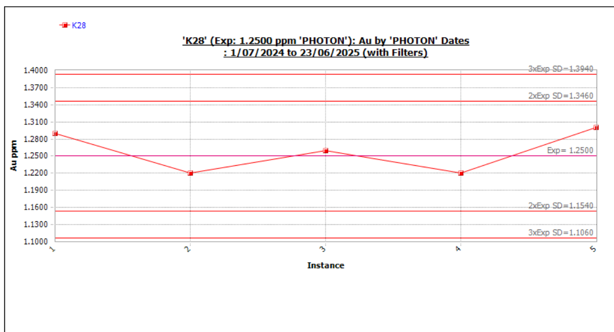
Figure 11-45 Standard K28 outliers included. Source: Westgold.
