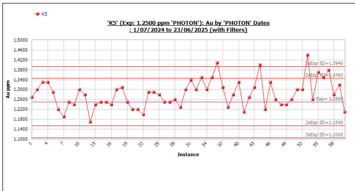
Figure 11-72 Standard K54 outliers included. Source: Westgold.
