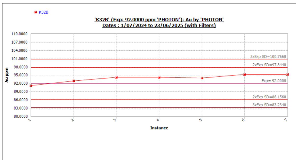
Figure 11-53 Standard K32B outliers included. Source: Westgold.
