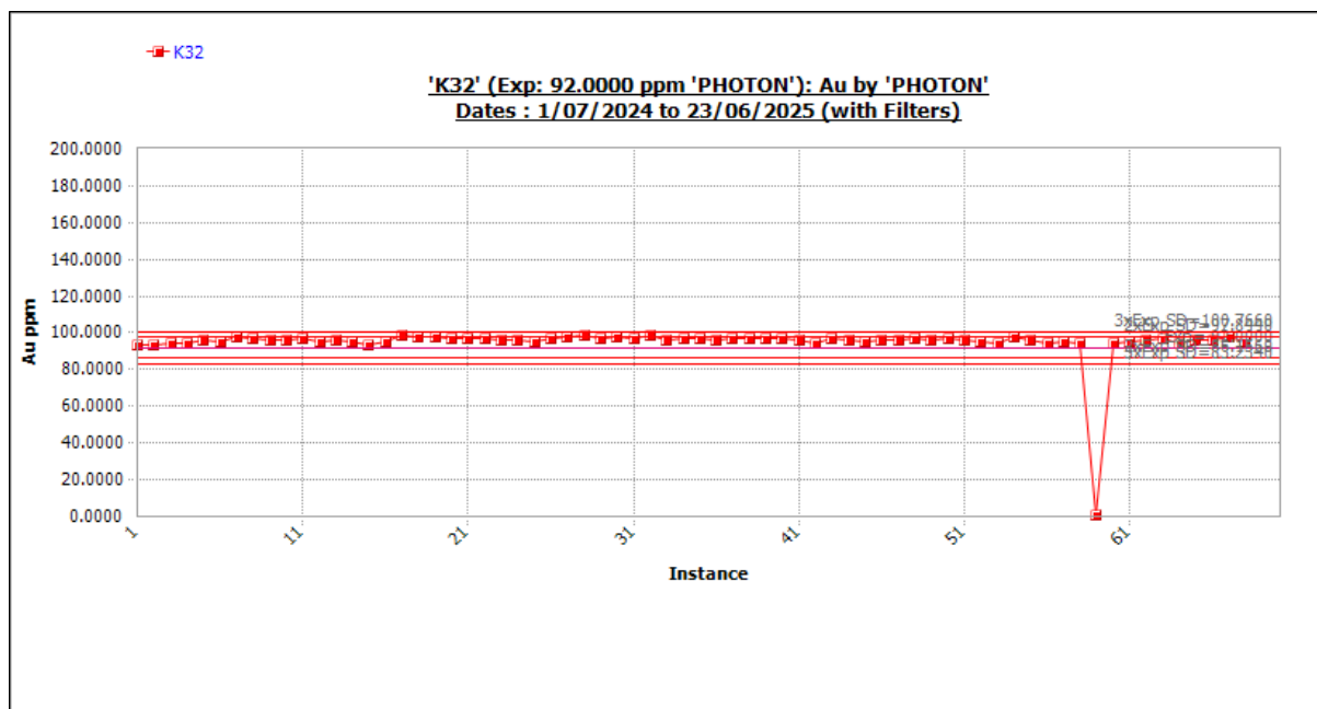
Figure 11-52 Standard K32 outliers included. Source: Westgold.
