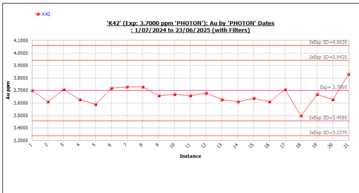
Figure 11-64 Standard K42 outliers included. Source: Westgold.
