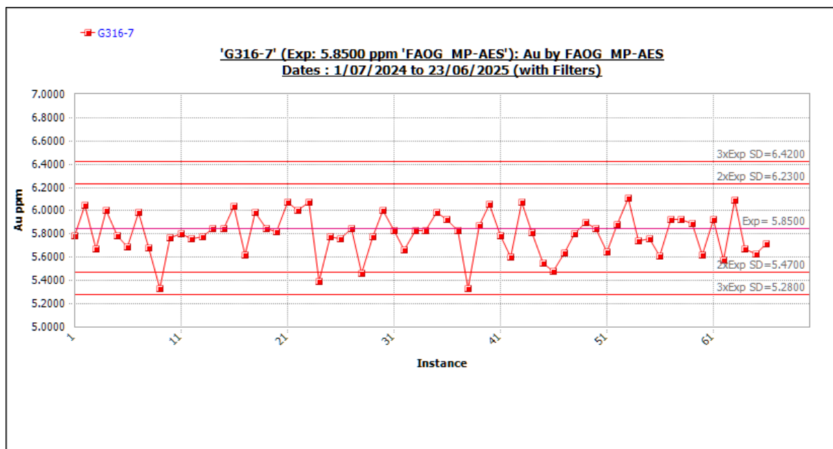
Figure 11-10 Standard G316-7 outliers included. Source: Westgold.
