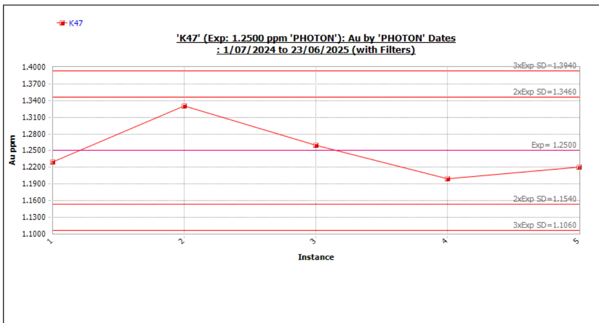
Figure 11-69 Standard K47 outliers included. Source: Westgold.
