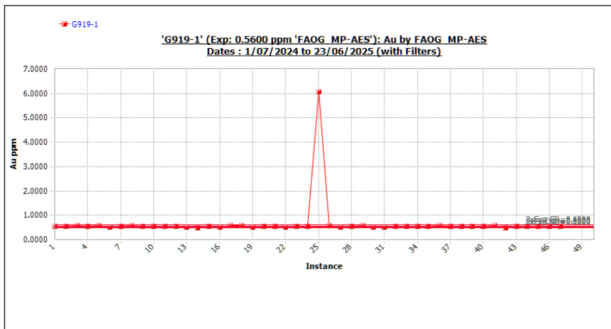
Figure 11-22 Standard G919-1 outliers included. Source: Westgold.
