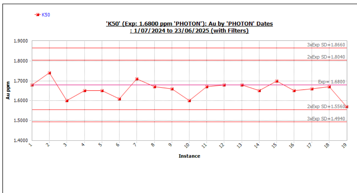
Figure 11-73 Standard K50 outliers included. Source: Westgold.
