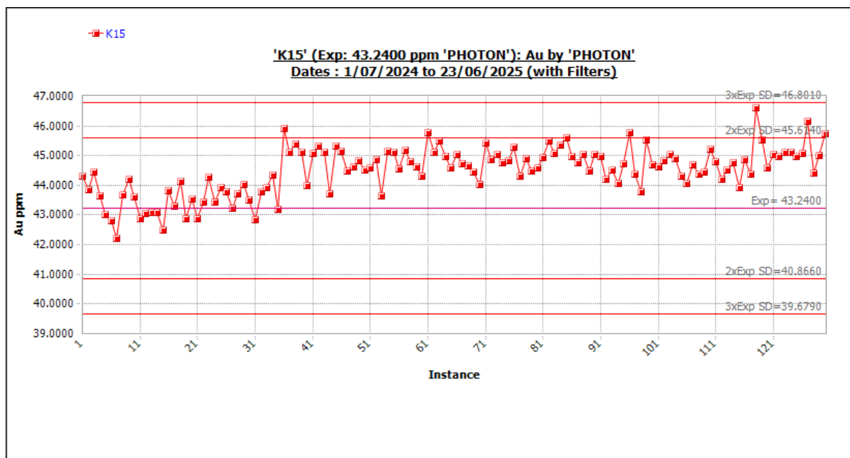
Figure 11-28 Standard K15 outliers included. Source: Westgold.
