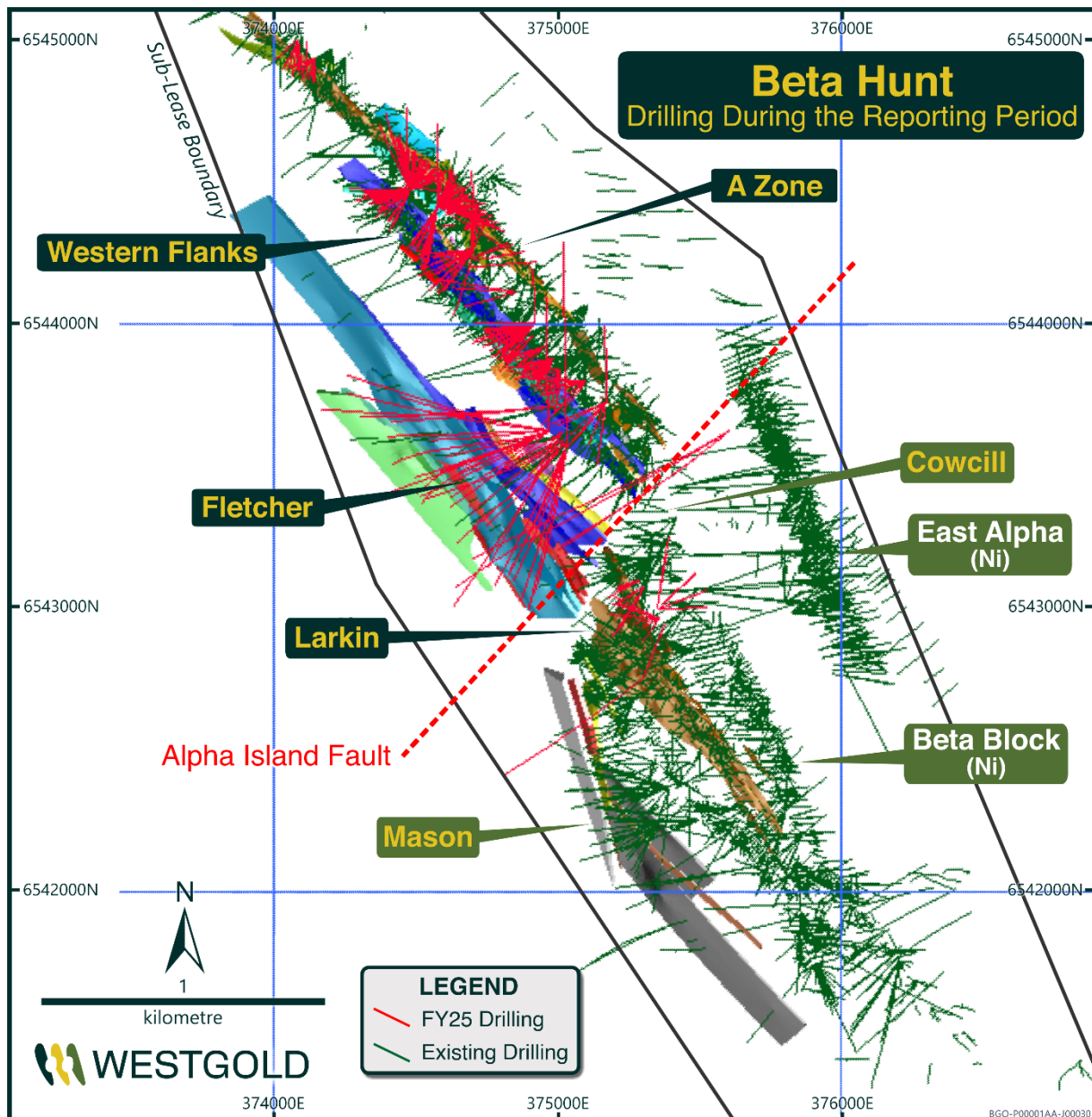
Figure 10-1 Plan highlights new drilling (magenta), 1 July 2024 to 23 June 2025, at Beta Hunt – Source : Westgold.
