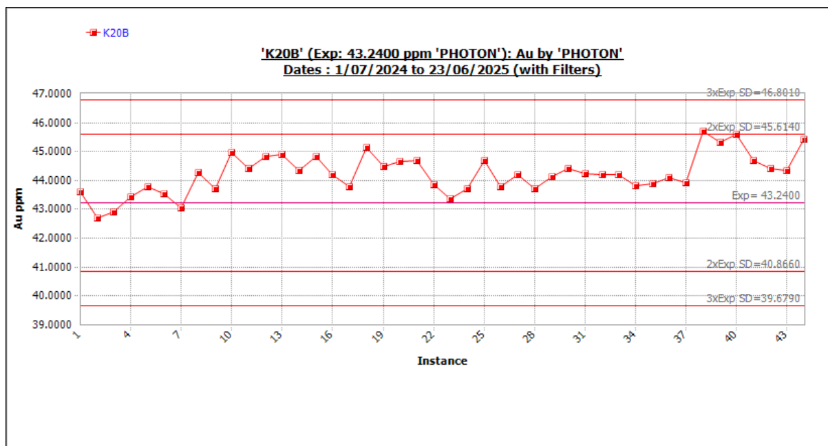
Figure 11-32 Standard K20B outliers included. Source: Westgold.
