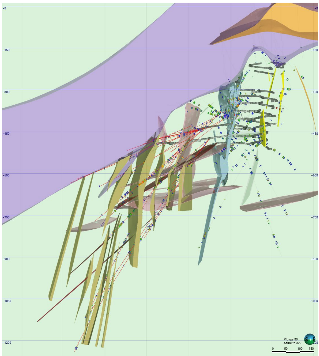
Figure 14-36 Example cross section of the geology model. Modelled lithology is mafic (green), ultramafic (purple), granodiorite (orange), porphyry (pink) and sediment (dark red). Mineralisation domains for Fletcher (brown), Western Flanks (aqua) and A-Zone (yellow) also shown. Drillholes intersecting the Fletcher mineralisation domains are red traces, with all drillhole assays above 0.3 g/t shown - Source : Westgold.
