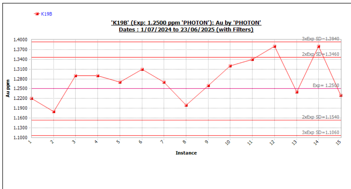
Figure 11-30 Standard K19B outliers included. Source: Westgold.
