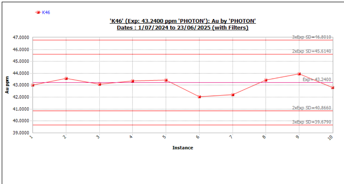
Figure 11-68 Standard K46 outliers included. Source: Westgold.
