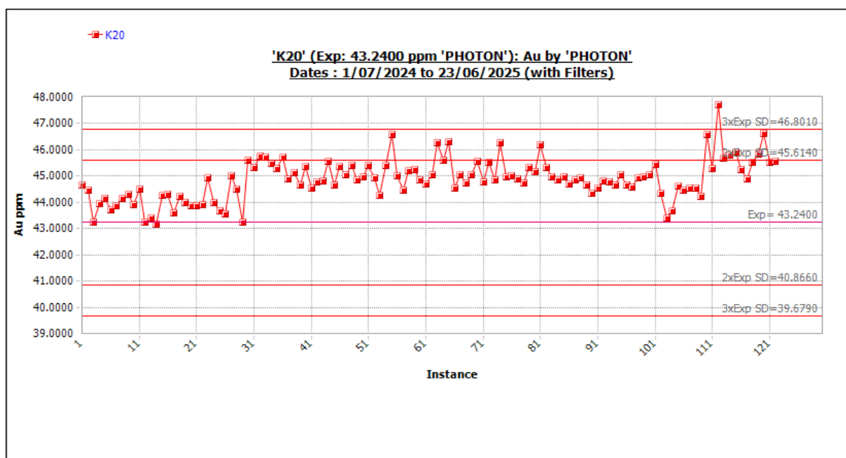
Figure 11-31 Standard K20 outliers included. Source: Westgold.
