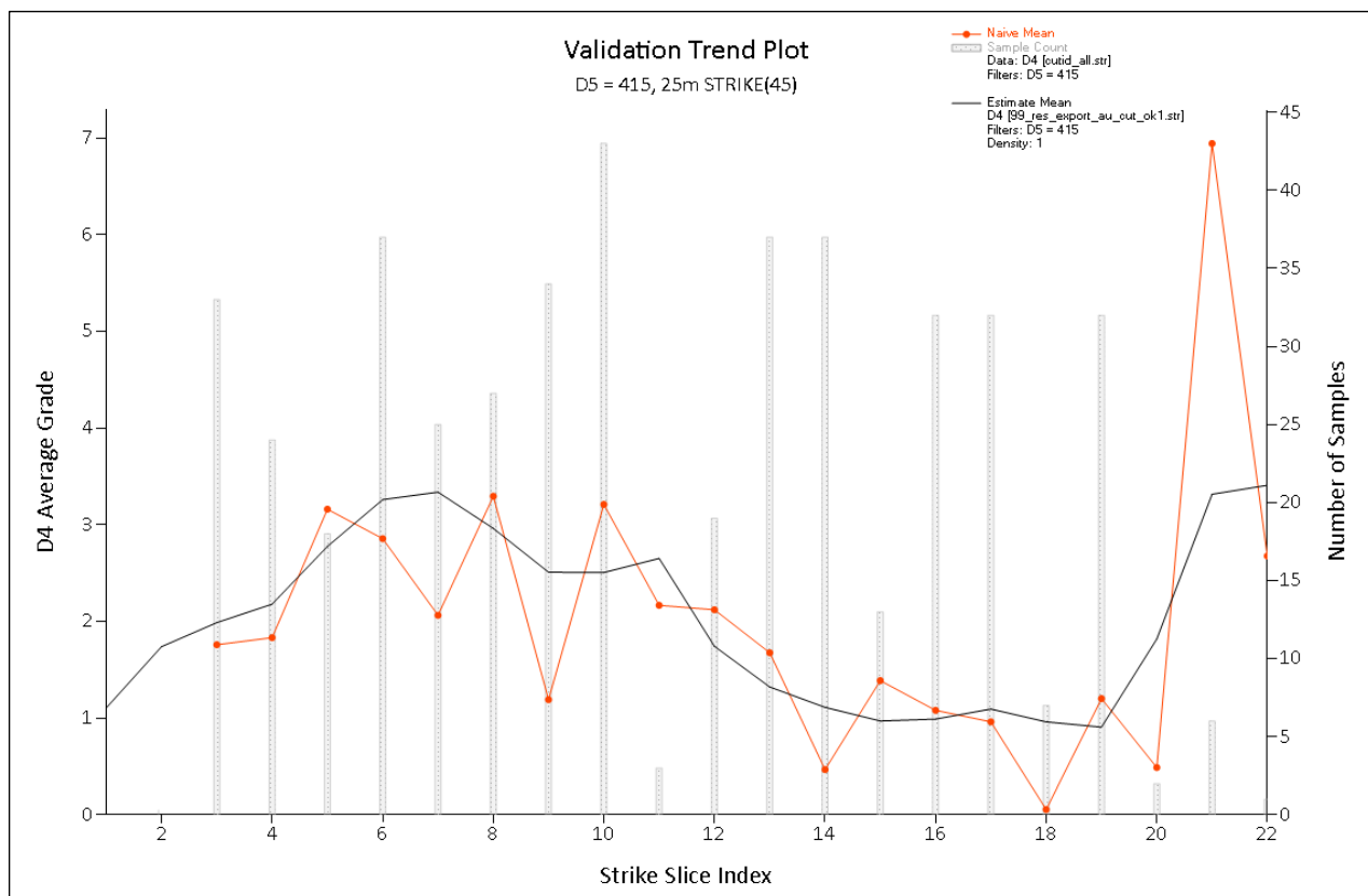
Figure 14-26 Trend swath plot for Domain 415 – along strike 45° - Source : Westgold.
