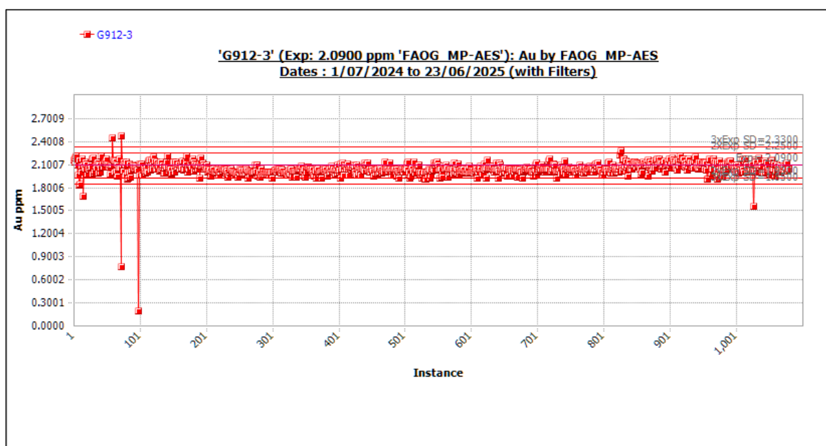
Figure 11-17 Standard G912-3 outliers included. Source: Westgold.
