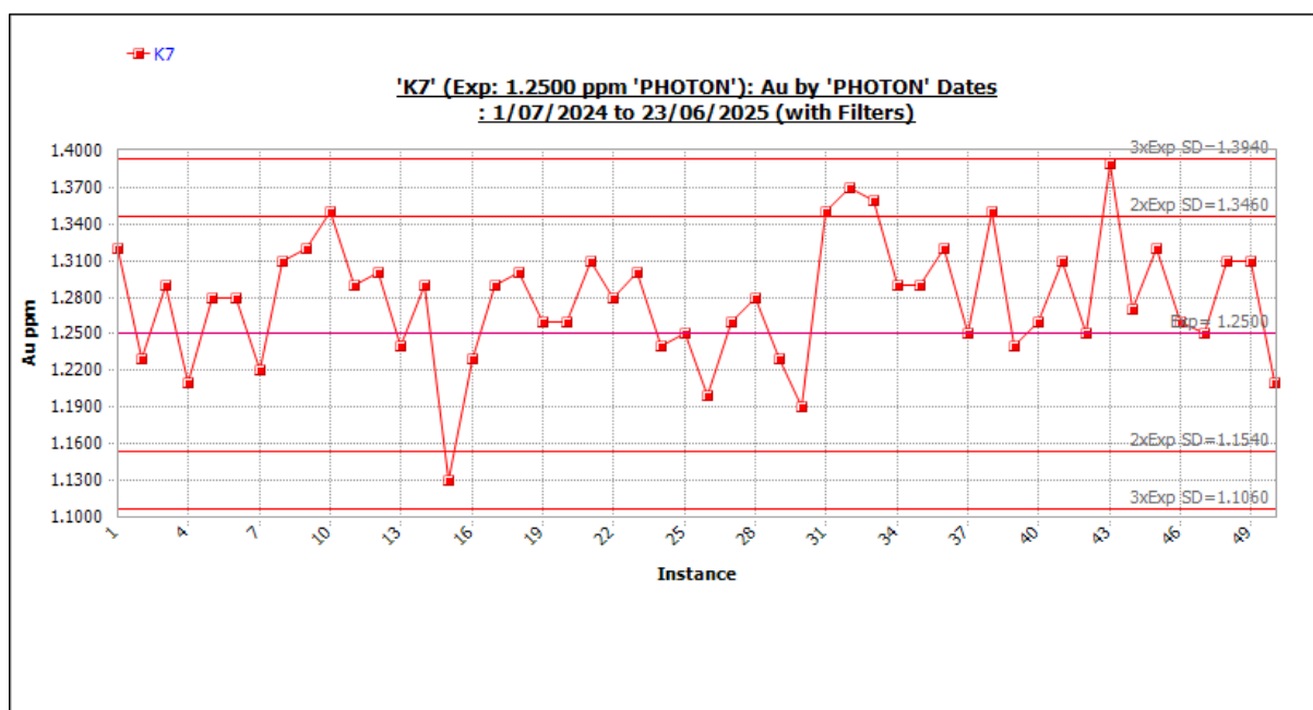
Figure 11-79 Standard K7 outliers included. Source: Westgold.
