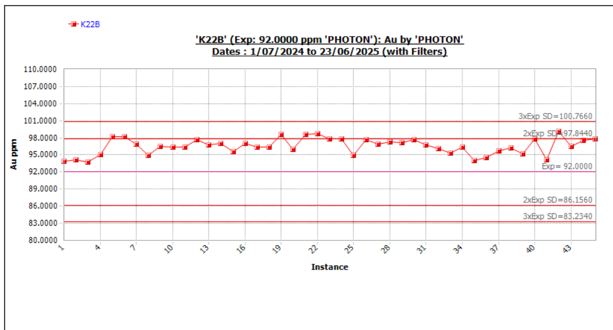
Figure 11-36 Standard K22B outliers included. Source: Westgold.
