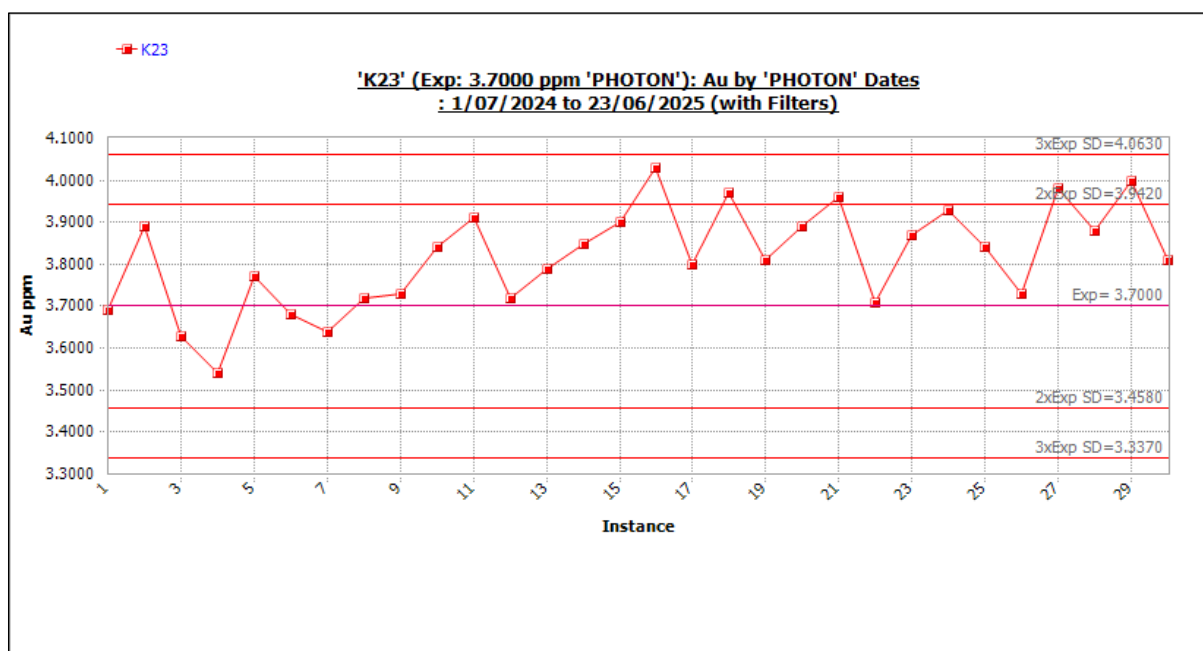
Figure 11-37 Standard K23 outliers included. Source: Westgold.
