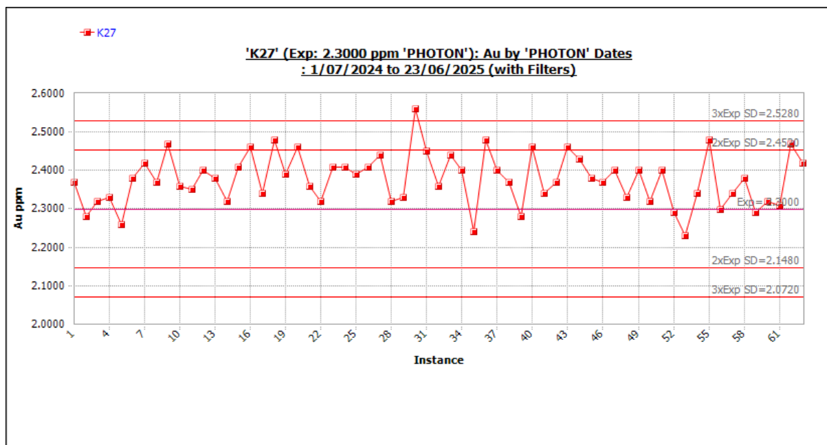
Figure 11-44 Standard K27 outliers included. Source: Westgold.
