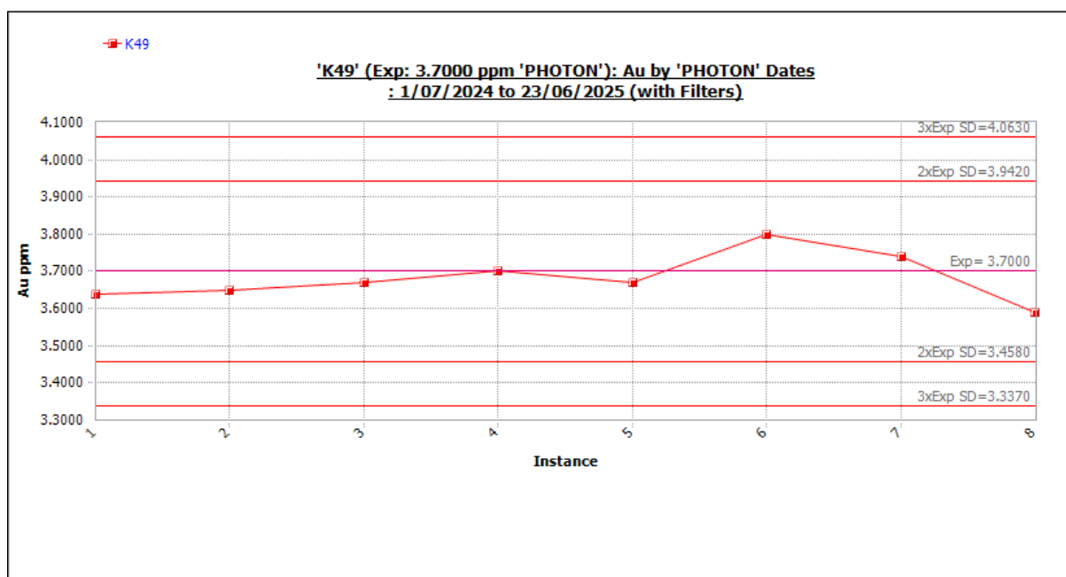
Figure 11-71 Standard K49 outliers included. Source: Westgold.
