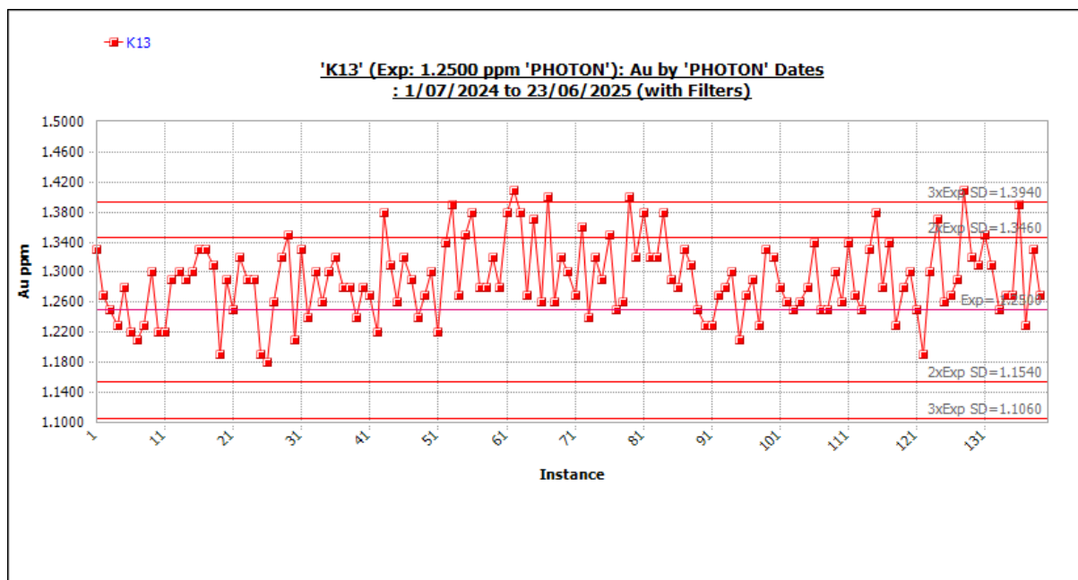
Figure 11-26 Standard K13 outliers included. Source: Westgold.
