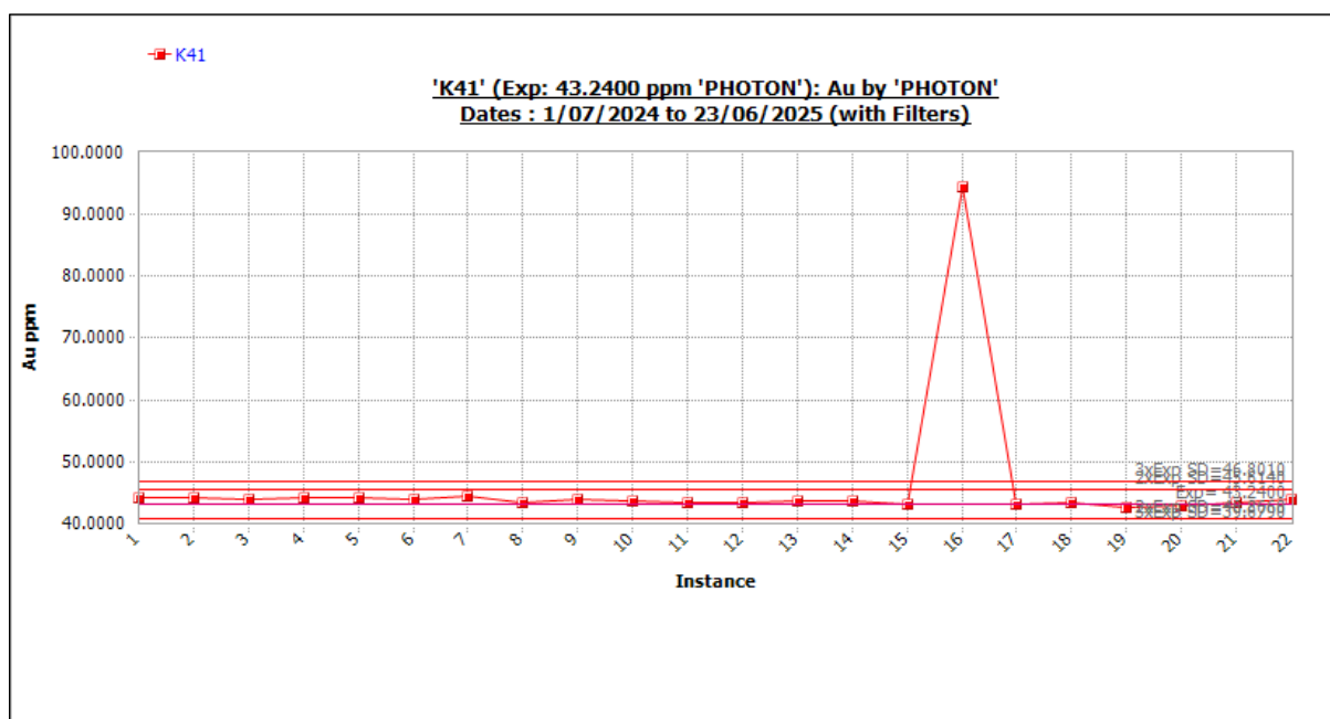
Figure 11-63 Standard K41 outliers included. Source: Westgold.
