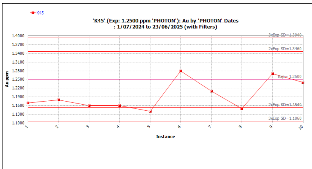
Figure 11-67 Standard K45 outliers included. Source: Westgold.
