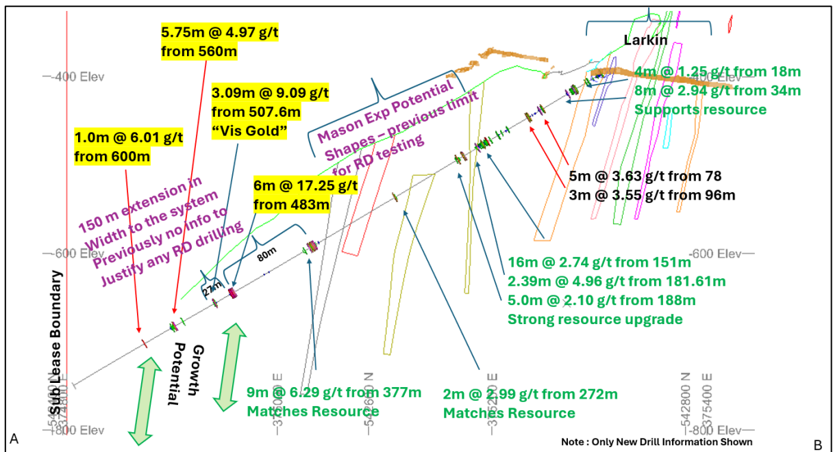
Figure 10-4 Section view showing the new hole which has proven significant western extensions to the Mason system. Relevant intersections outside the mineral potential model are highlighted in yellow – Source : Westgold.
