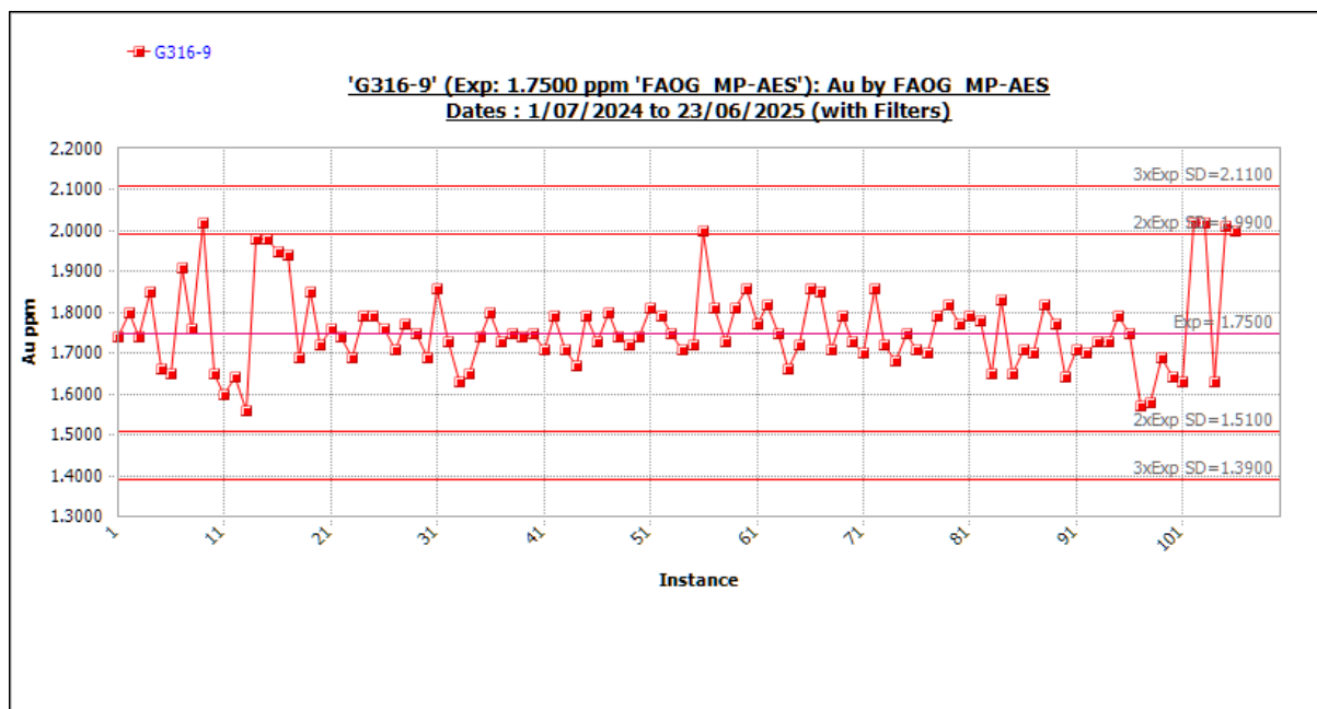
Figure 11-12 Standard G316-9 outliers included. Source: Westgold.
