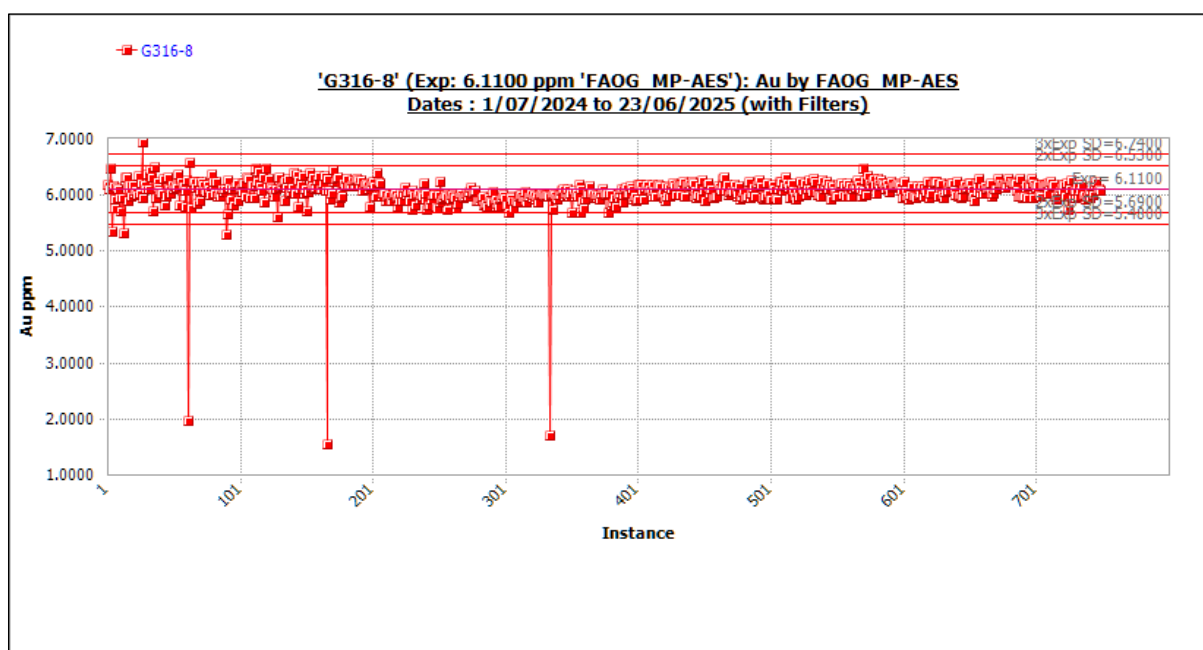
Figure 11-11 Standard G316-8 outliers included. Source: Westgold.
