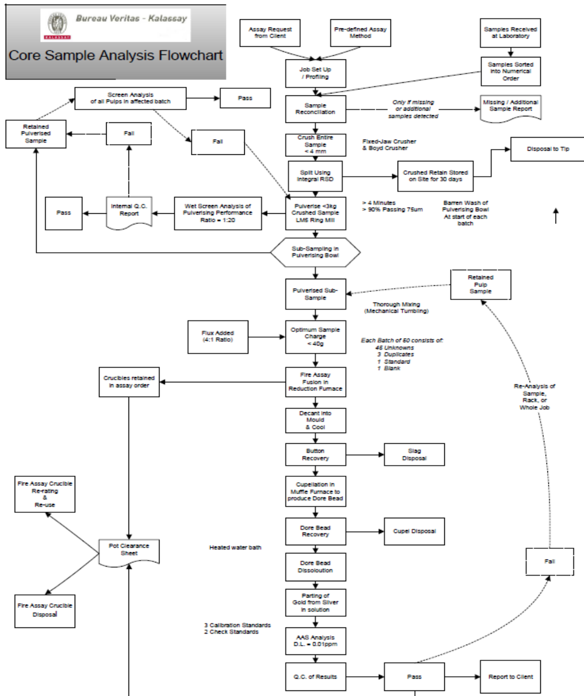
Figure 11-1 Representative fire assay sample flow chart Bureau Veritas. Source: Westgold.
