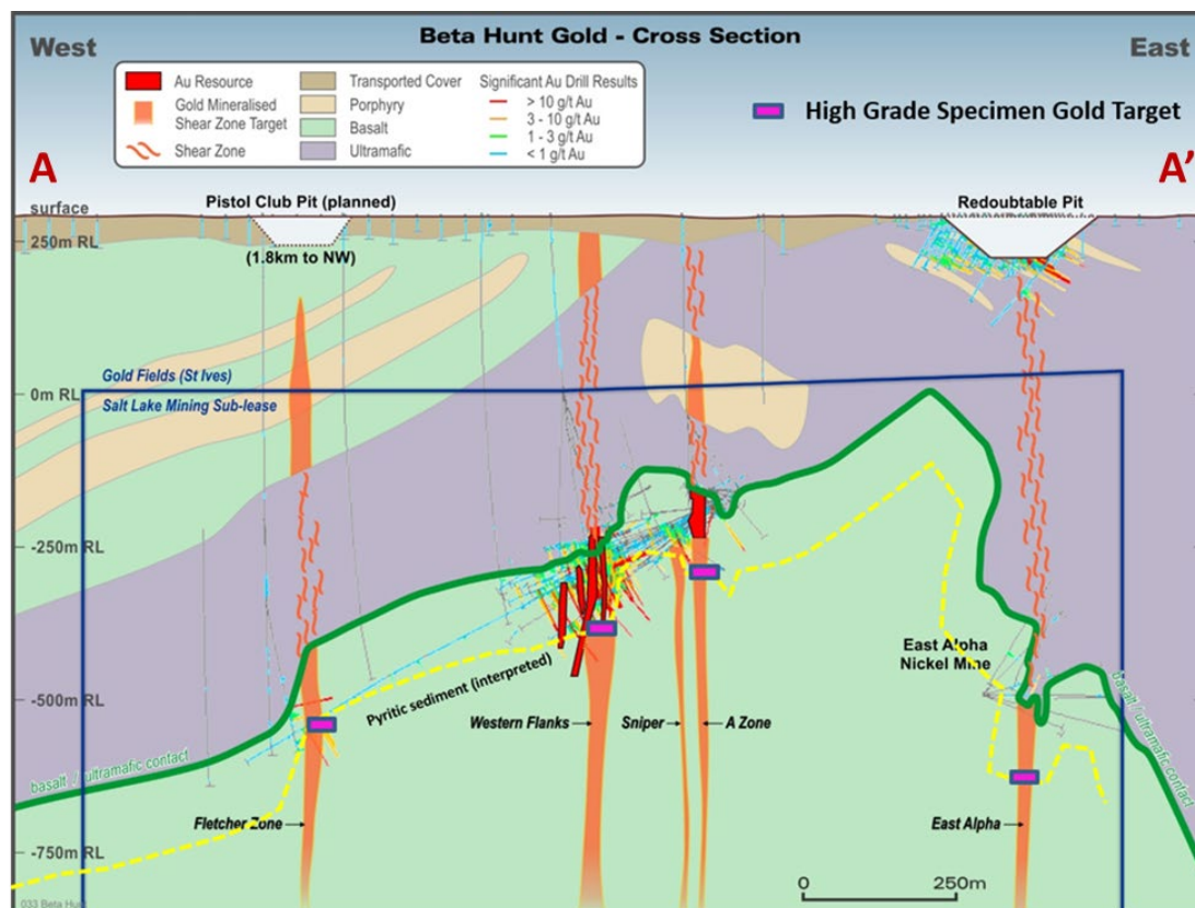
Figure 7-6 Composite cross-section looking north showing interpreted shear zone related gold mineralisation and rock type Source : Westgold.
