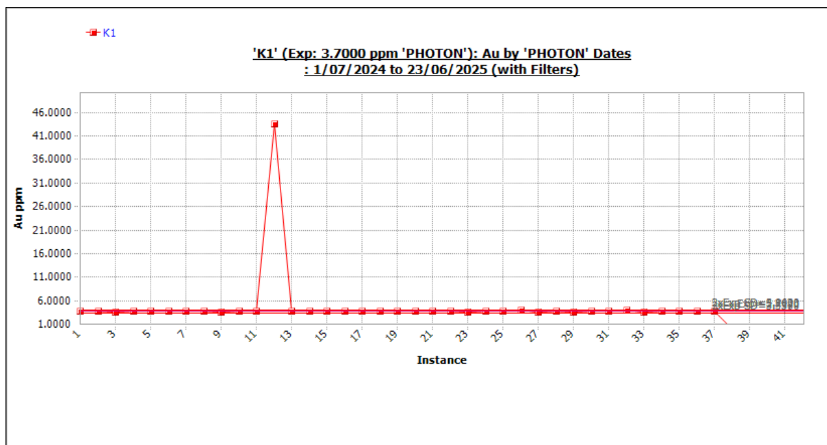
Figure 11-24 Standard K1 outliers included. Source: Westgold.
