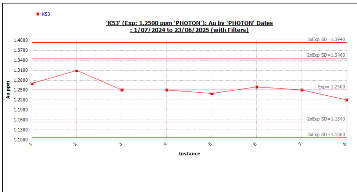
Figure 11-76 Standard K53 outliers included. Source: Westgold.
