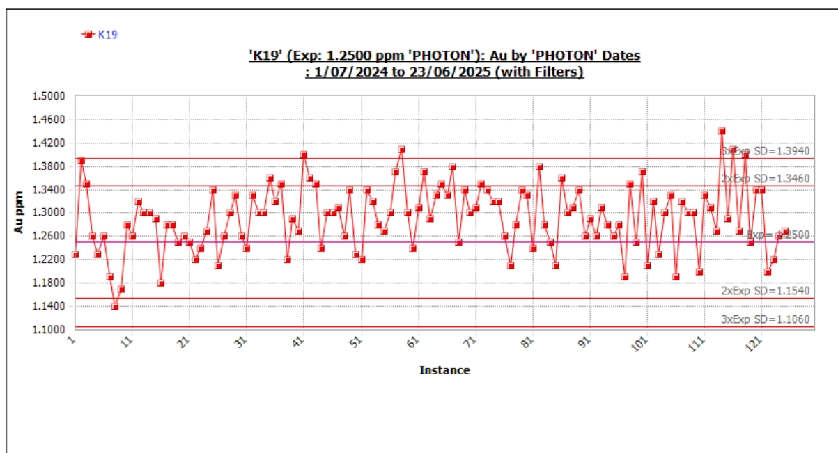
Figure 11-29 Standard K19 outliers included. Source: Westgold.
