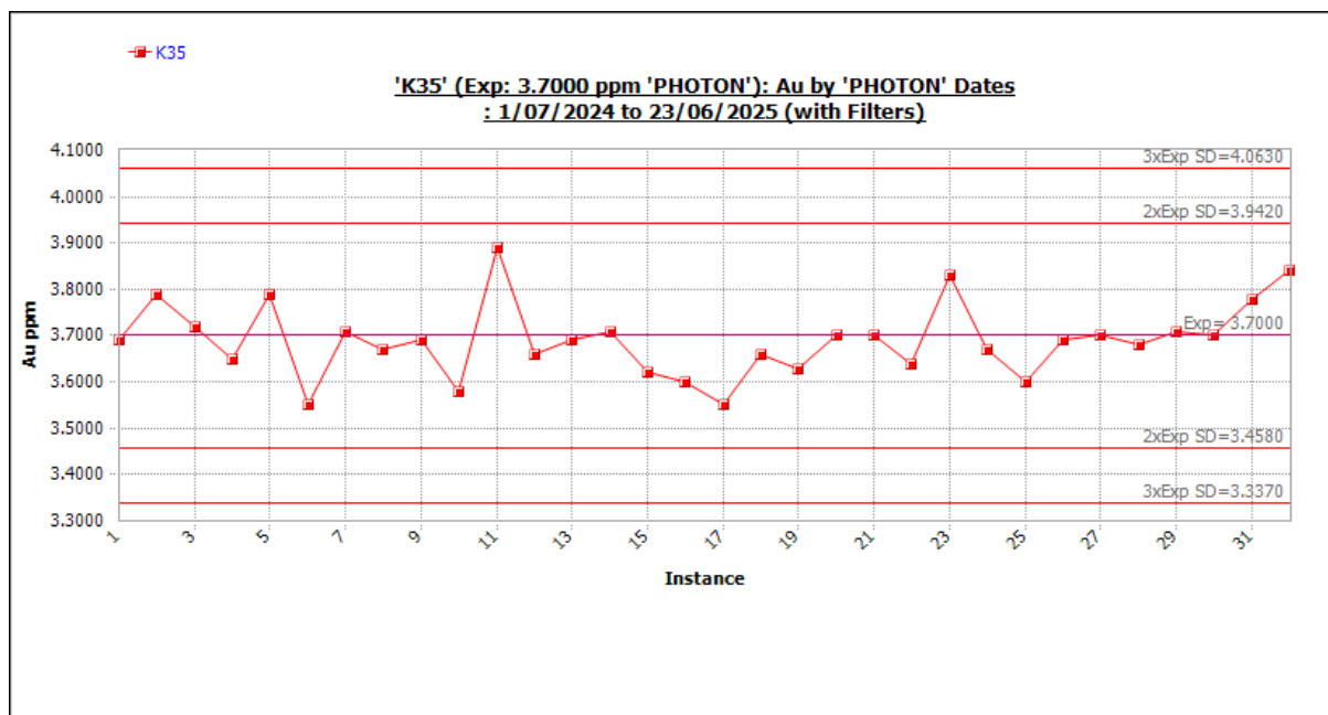
Figure 11-56 Standard K35 outliers included. Source: Westgold.
