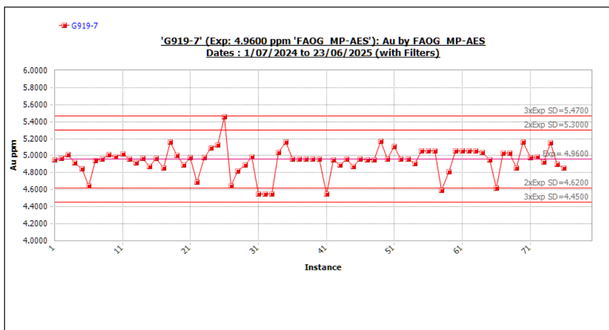
Figure 11-23 Standard G919-7 outliers included. Source: Westgold.
