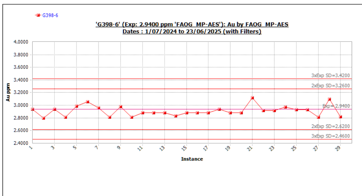
Figure 11-15 Standard G398-6 outliers included. Source: Westgold.
