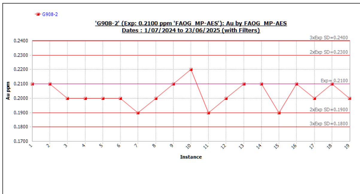
Figure 11-16 Standard G908-2 outliers included. Source: Westgold.
