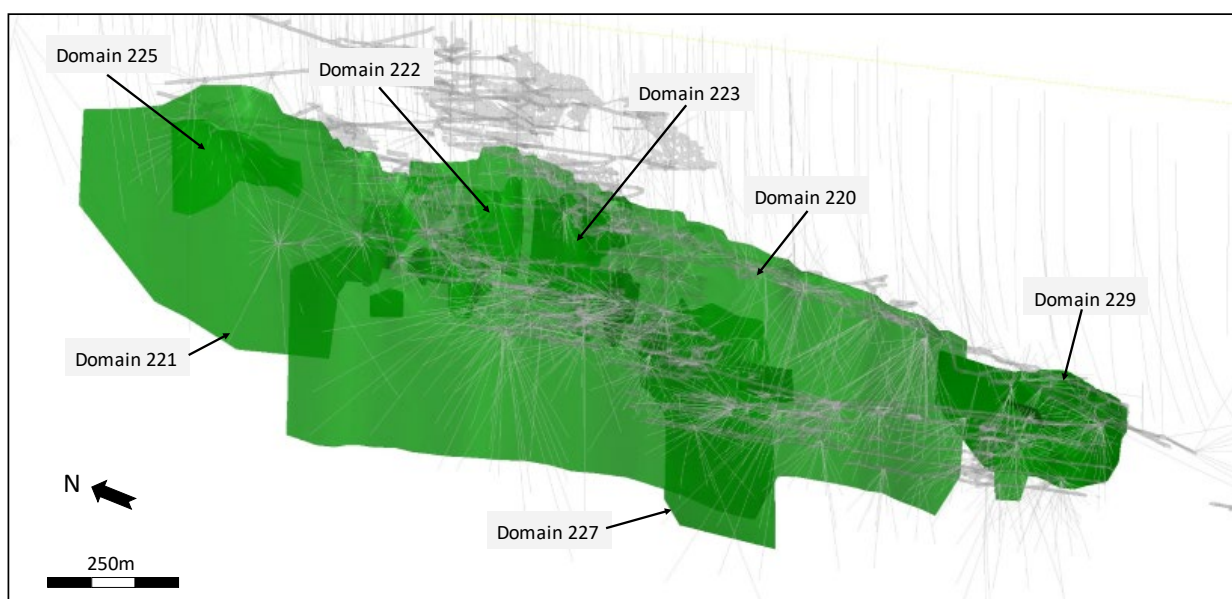
Figure 14-4 A Zone main mineralisation wireframes – oblique view looking east-northeast – Source : Westgold.
