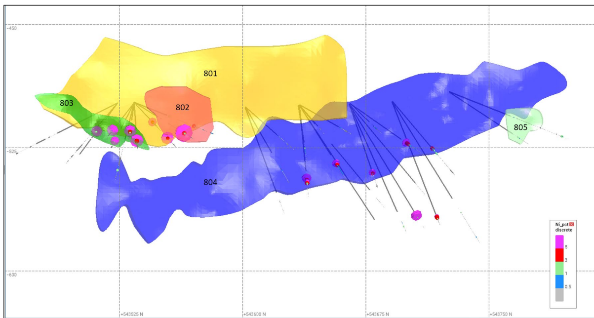
Figure 14-43 Isometric view of Kappa and Delta lenses, looking west, showing the infill drill holes only with Ni grade – Source : Westgold.
