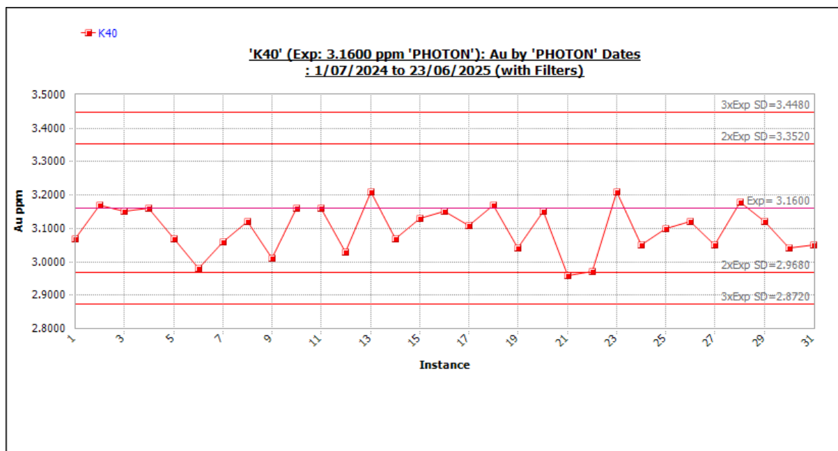
Figure 11-62 Standard K40 outliers included. Source: Westgold.
