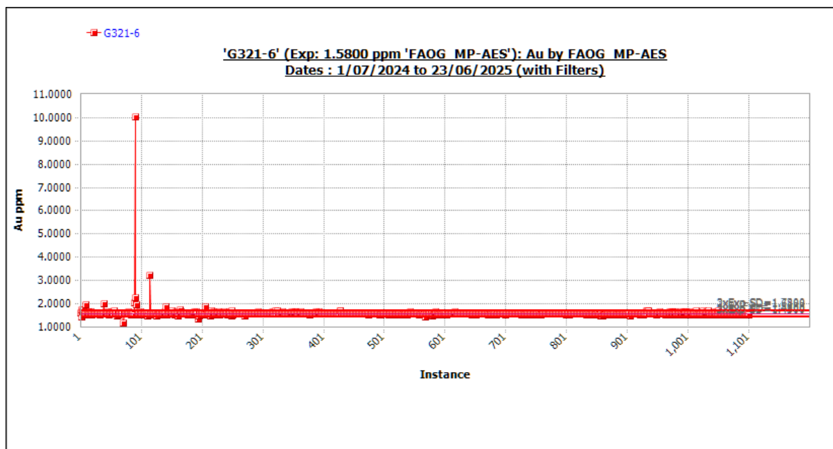
Figure 11-14 Standard G321-6 outliers included. Source: Westgold.
