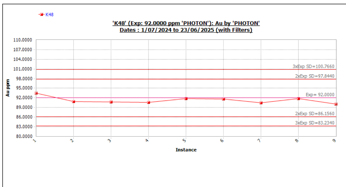
Figure 11-70 Standard K48 outliers included. Source: Westgold.
