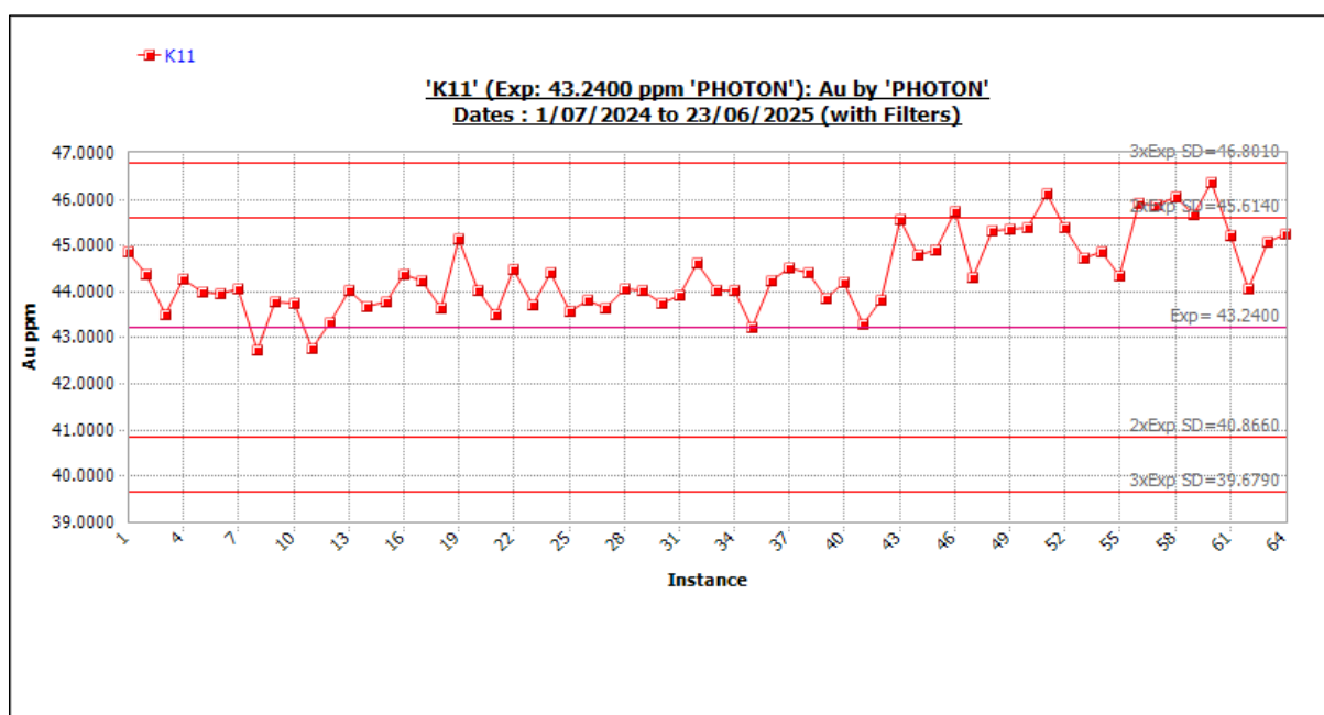
Figure 11-25 Standard K11 outliers included. Source: Westgold.
