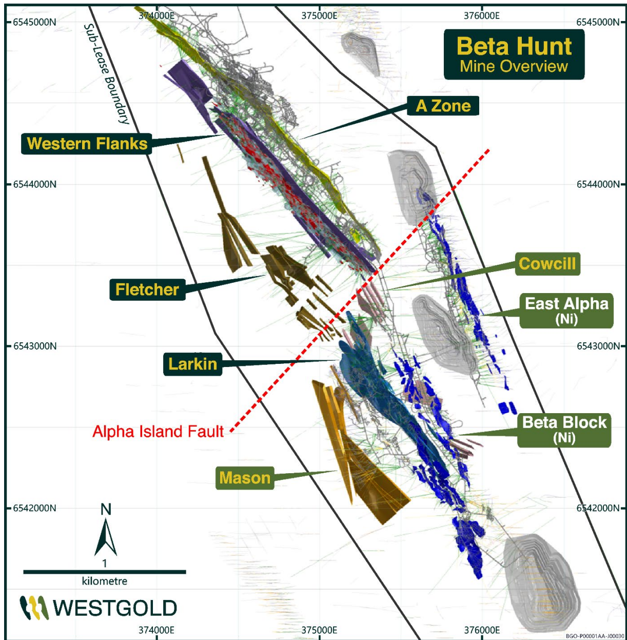
Figure 14-40 Beta Hunt Gold Mineral Resource Location Plan – Source : Westgold.
