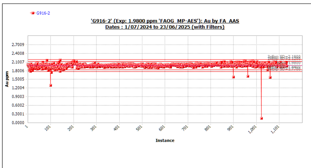
Figure 11-19 Standard G916-2 outliers included. Source: Westgold.
