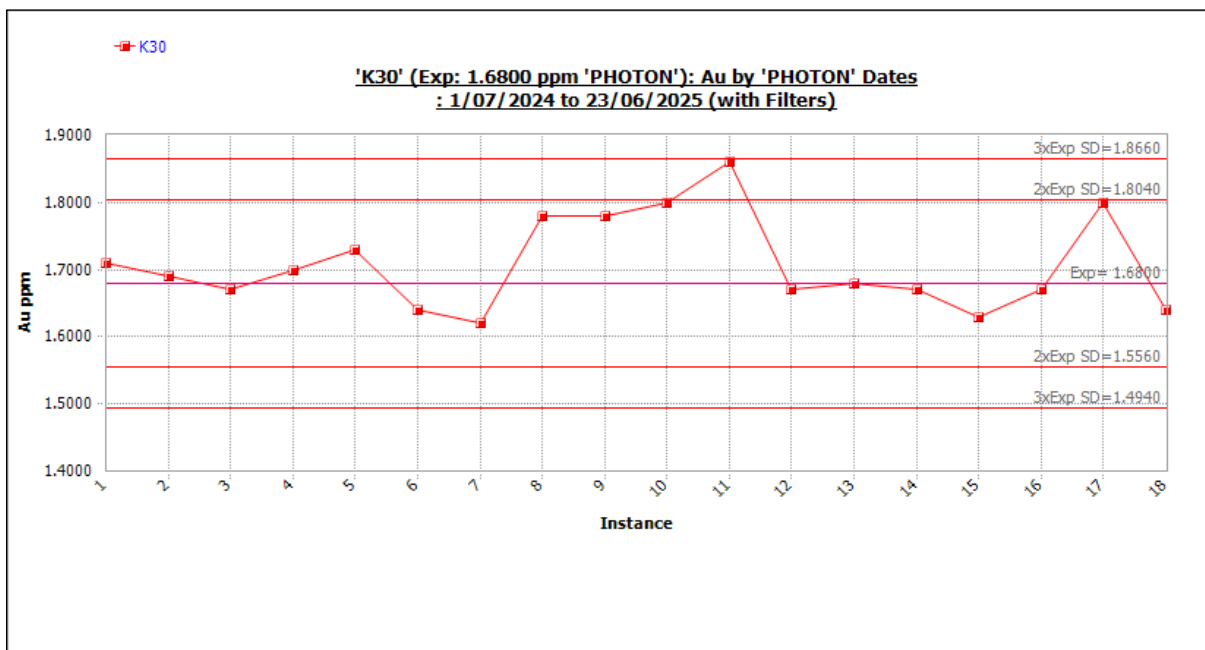
Figure 11-49 Standard K30 outliers included. Source: Westgold.
