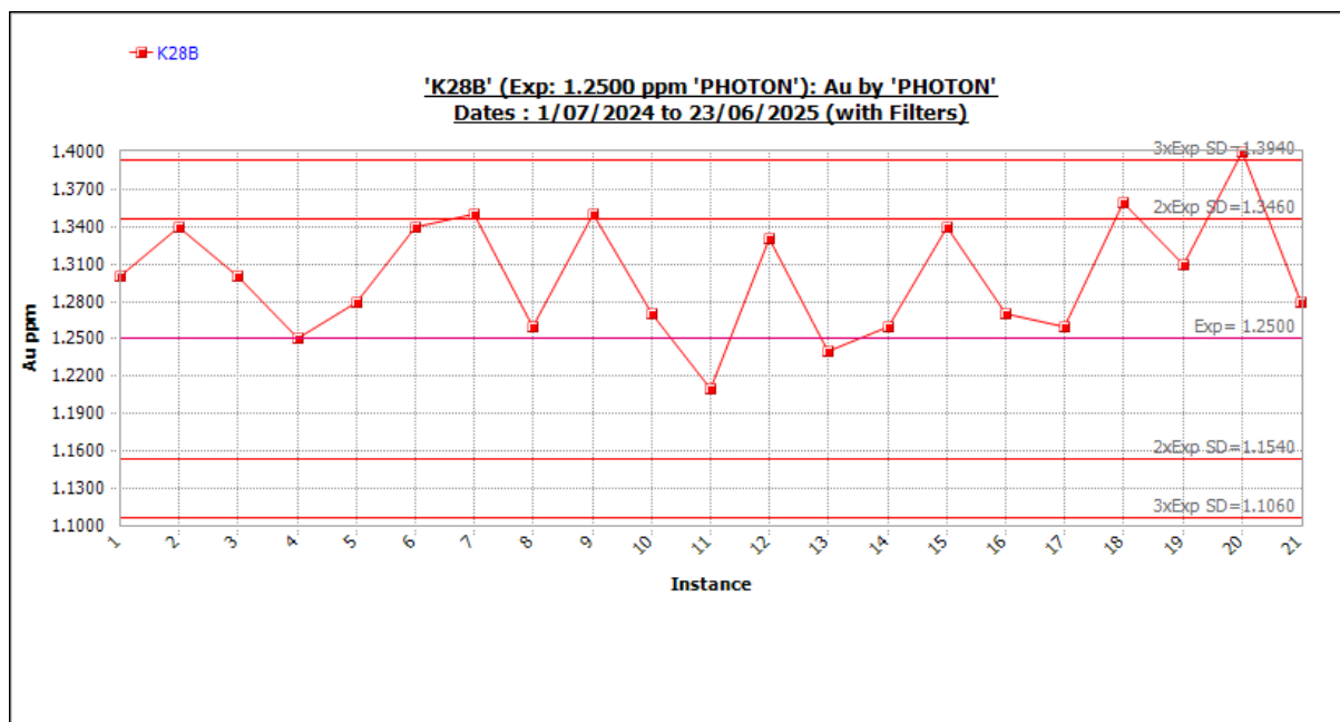
Figure 11-46 Standard K28B outliers included. Source: Westgold.
