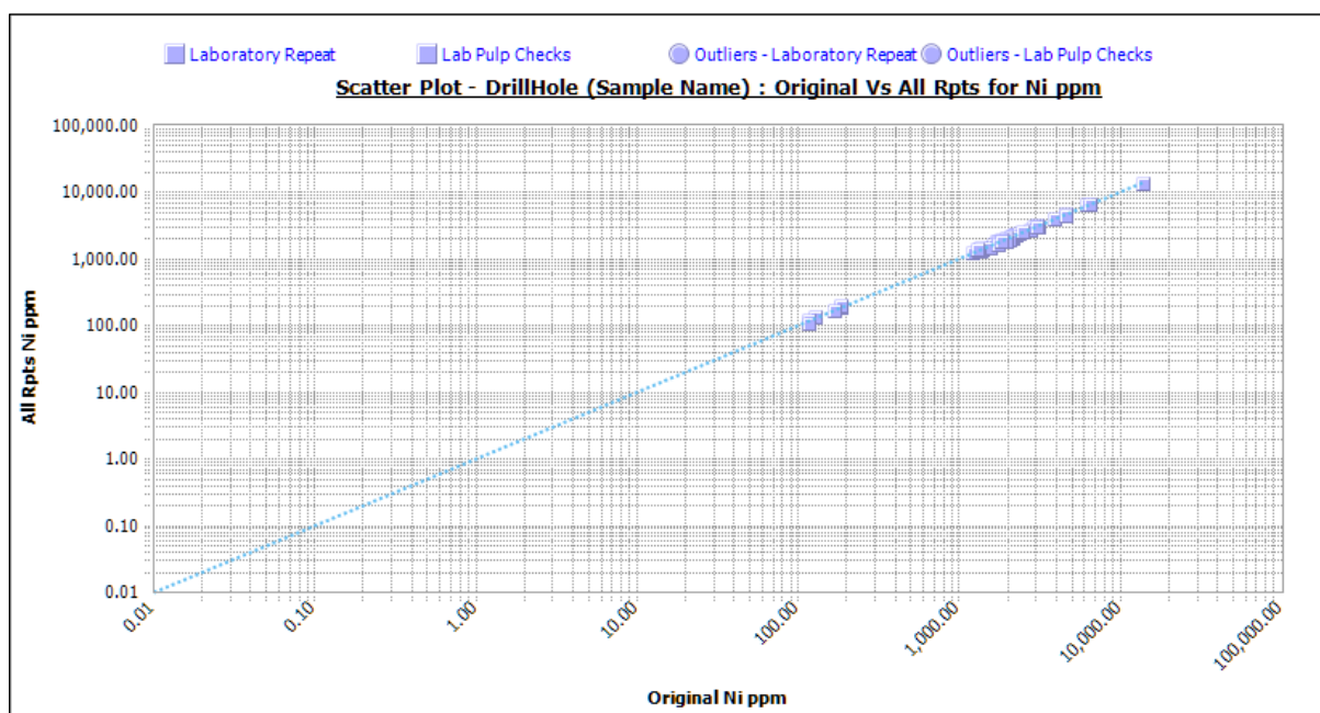
Figure 11-91 Scatter plot – DrillHole (sample name) original vs all repeats for Ni ppm. Source: Westgold.
