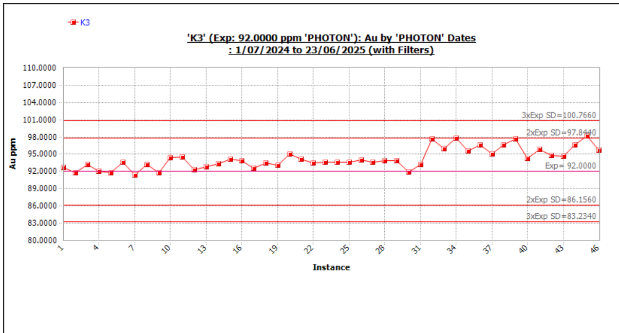
Figure 11-48 Standard K3 outliers included. Source: Westgold.
