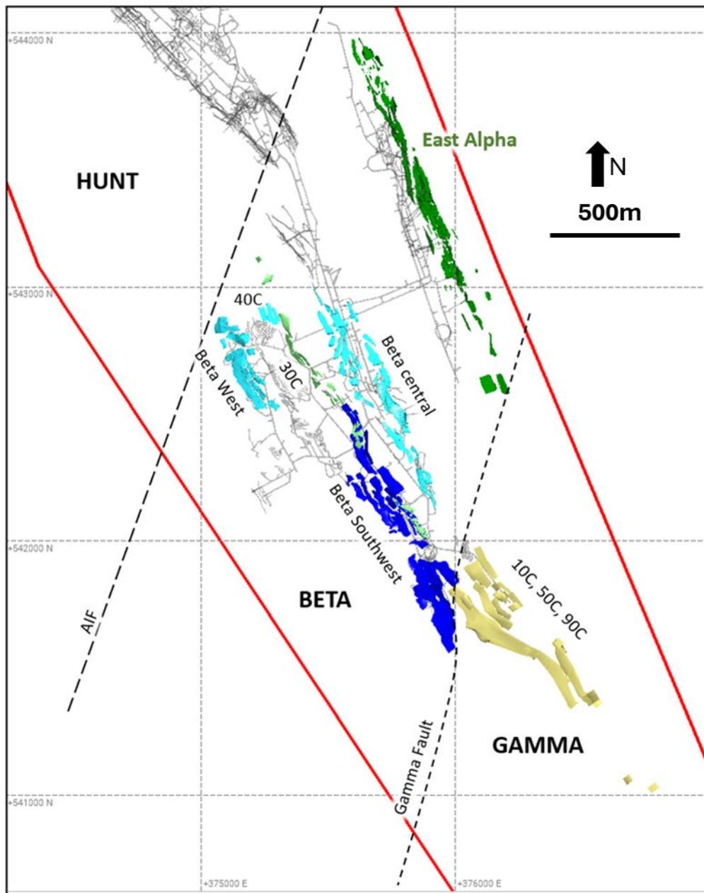
Figure 14-41 Beta Hunt June 2024 Nickel Mineral Resource locations – Source: Westgold.
