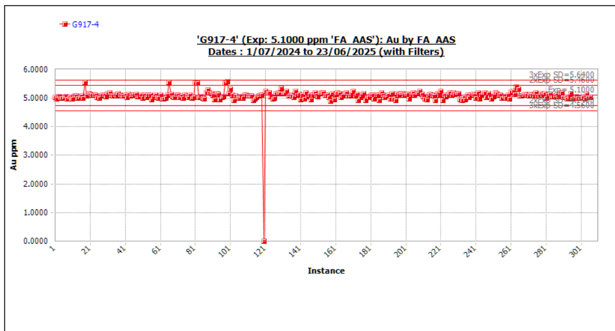
Figure 11-20 Standard G917-4 outliers included. Source: Westgold.
