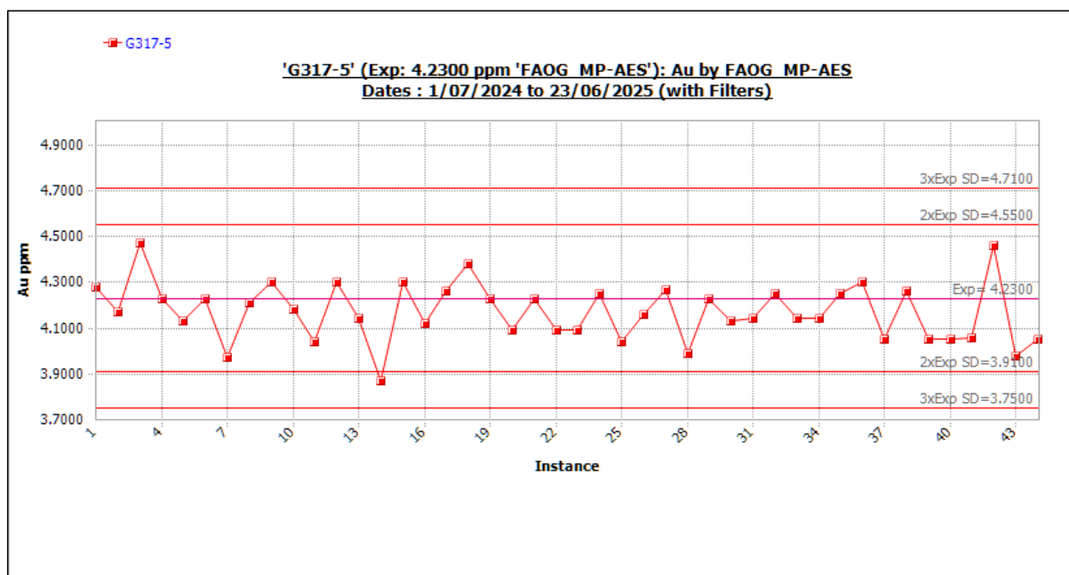
Figure 11-13 Standard G317-5 outliers included. Source: Westgold.
