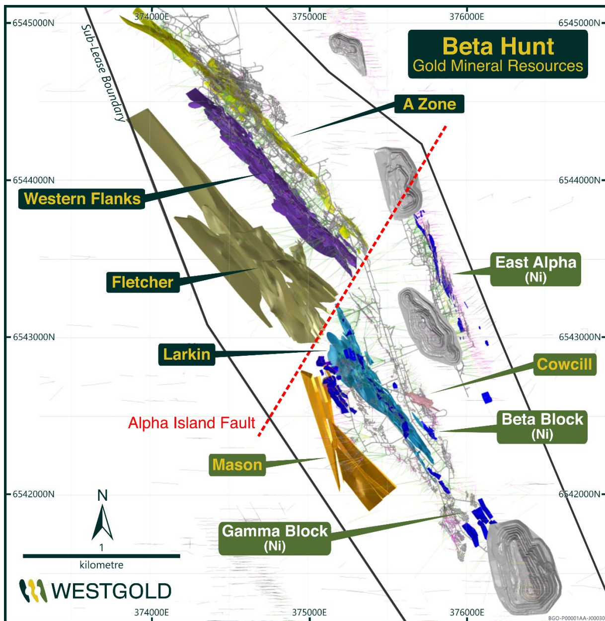
Figure 7-5 Plan view of 2025 gold and nickel Mineral Resources Source : Westgold.
