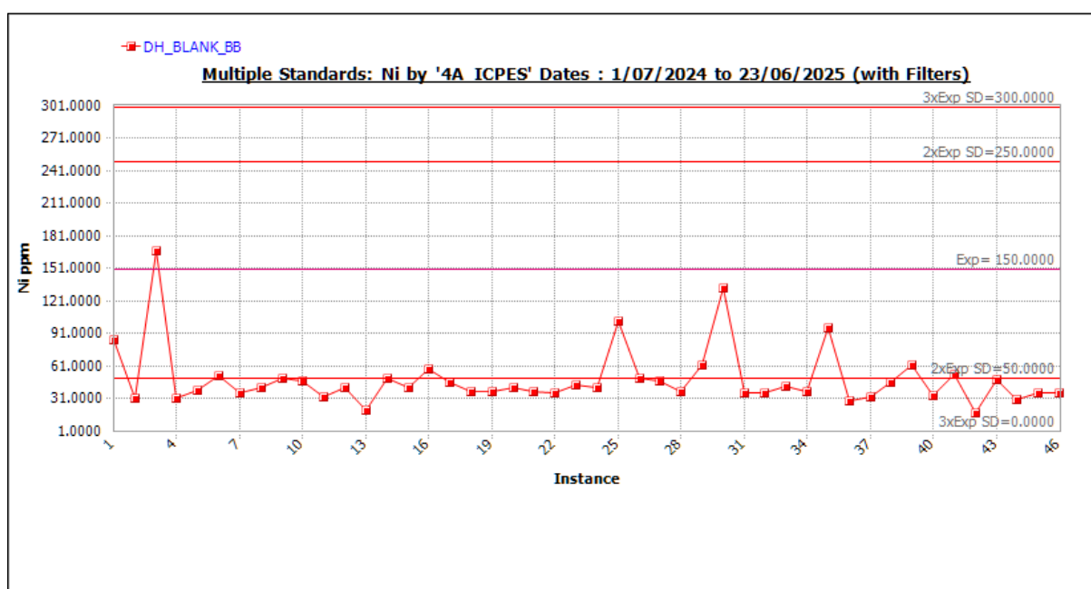
Figure 11-85 Standard DH_BLANK_BB. Source: Westgold.
