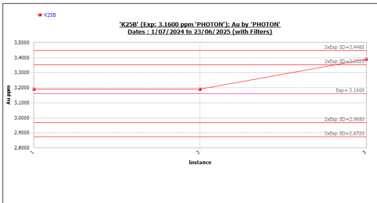
Figure 11-42 Standard K25B outliers included. Source: Westgold.
