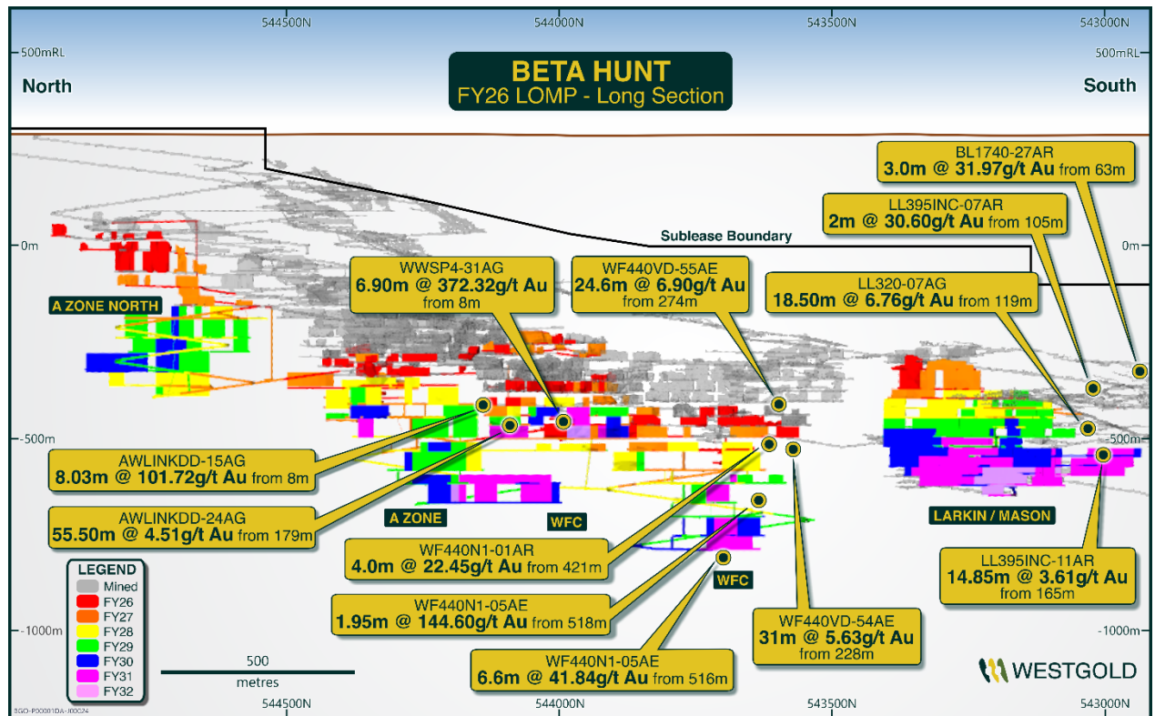
Figure 10-2 Beta Hunt schematic long-section showing select better results returned during the period 1 July 2024, through 23 June 2025 – Source : Westgold.
