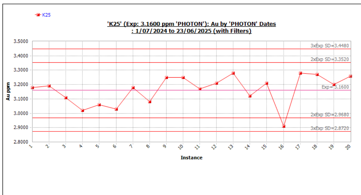
Figure 11-41 Standard K25 outliers included. Source: Westgold.
