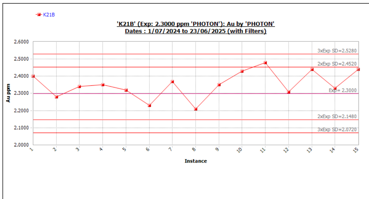
Figure 11-34 Standard K21B outliers included. Source: Westgold.
