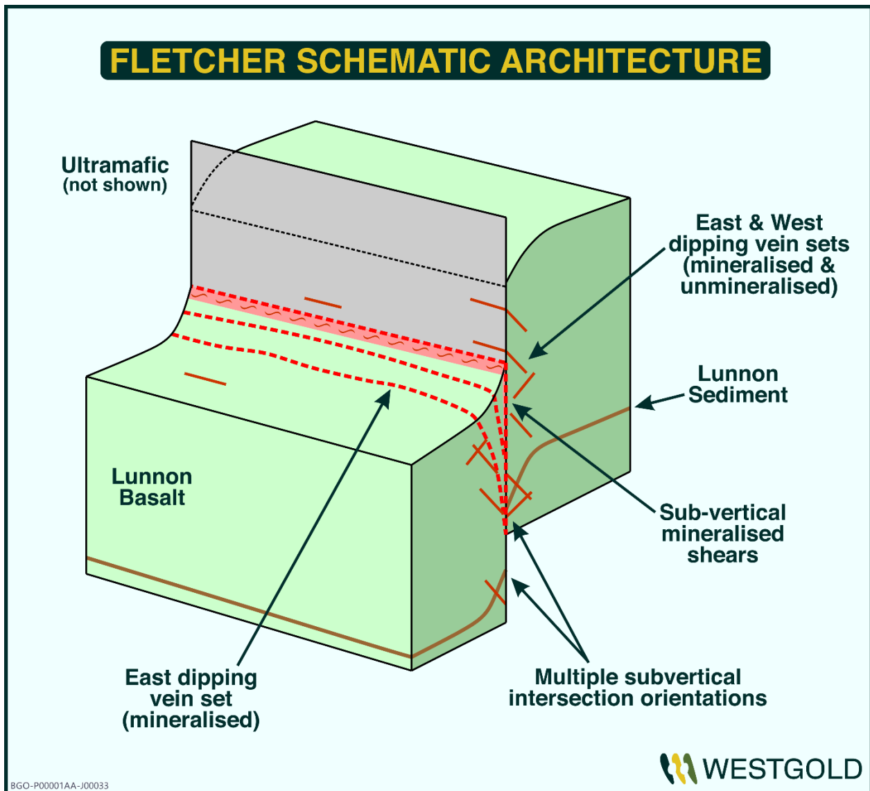
Figure 7-13 Mineralisation styles A Zone compared to Western Flanks – Source : Westgold Resources.
