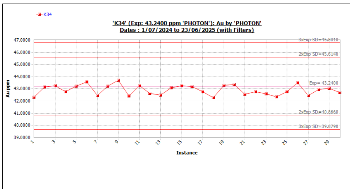
Figure 11-55 Standard K34 outliers included. Source: Westgold.
