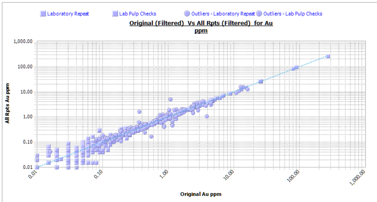
Figure 11-82 Scatter plot Fire Assay - drillhole (repeat code) : original vs all repeats for Au ppm. Source: Westgold.
