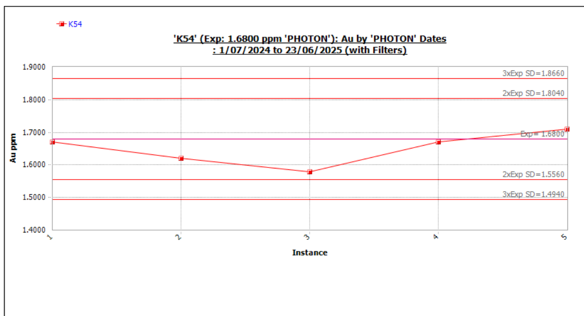
Figure 11-77 Standard K54 outliers included. Source: Westgold.
