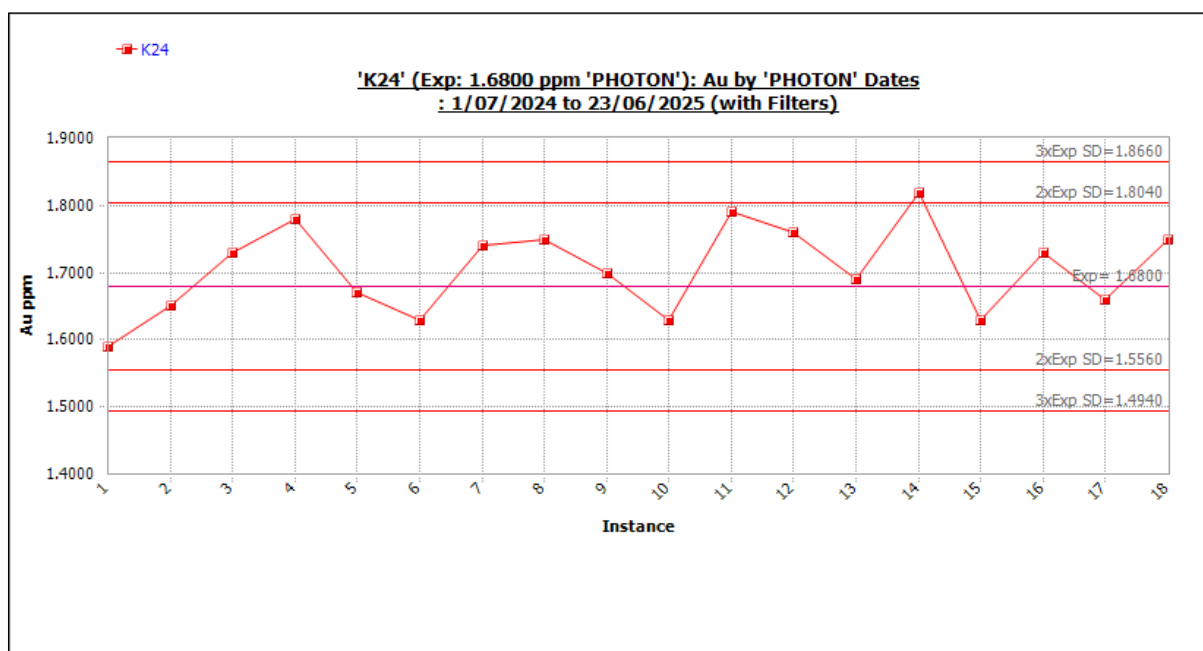
Figure 11-39 Standard K24 outliers included. Source: Westgold.
