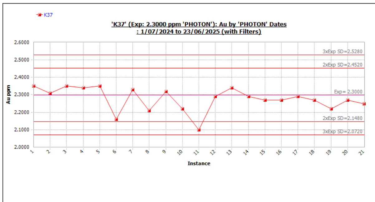
Figure 11-58 Standard K37 outliers included. Source: Westgold.
