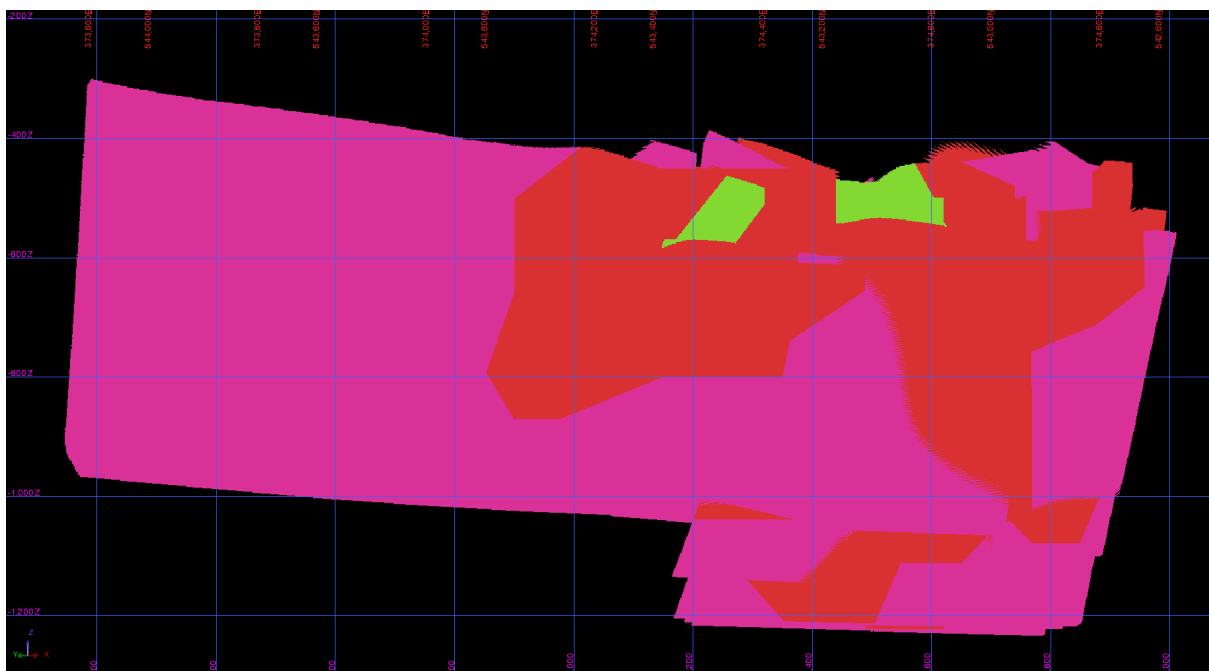
Figure 14-39 Fletcher Mineral Resource Classification, all mineralisation domains. Green = Indicated, red = Inferred, magenta is unreported material - Source : Westgold.
