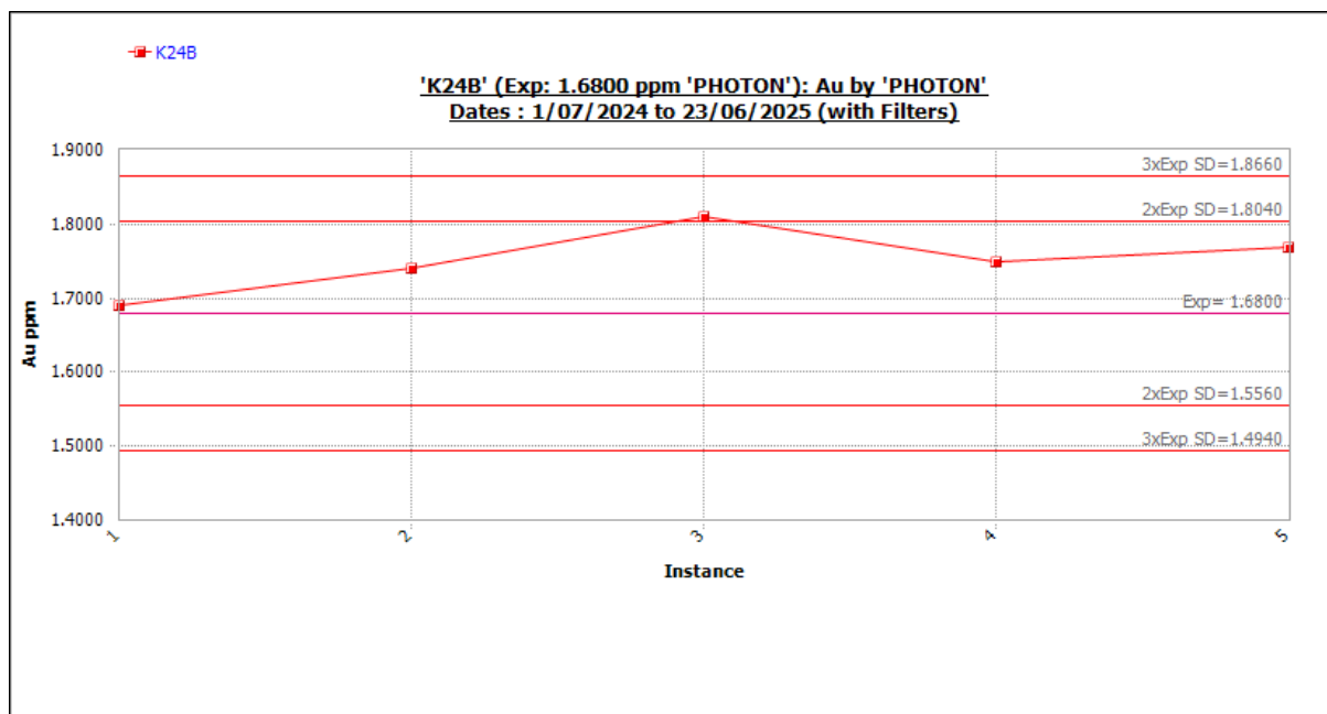
Figure 11-40 Standard K24B outliers included. Source: Westgold.
