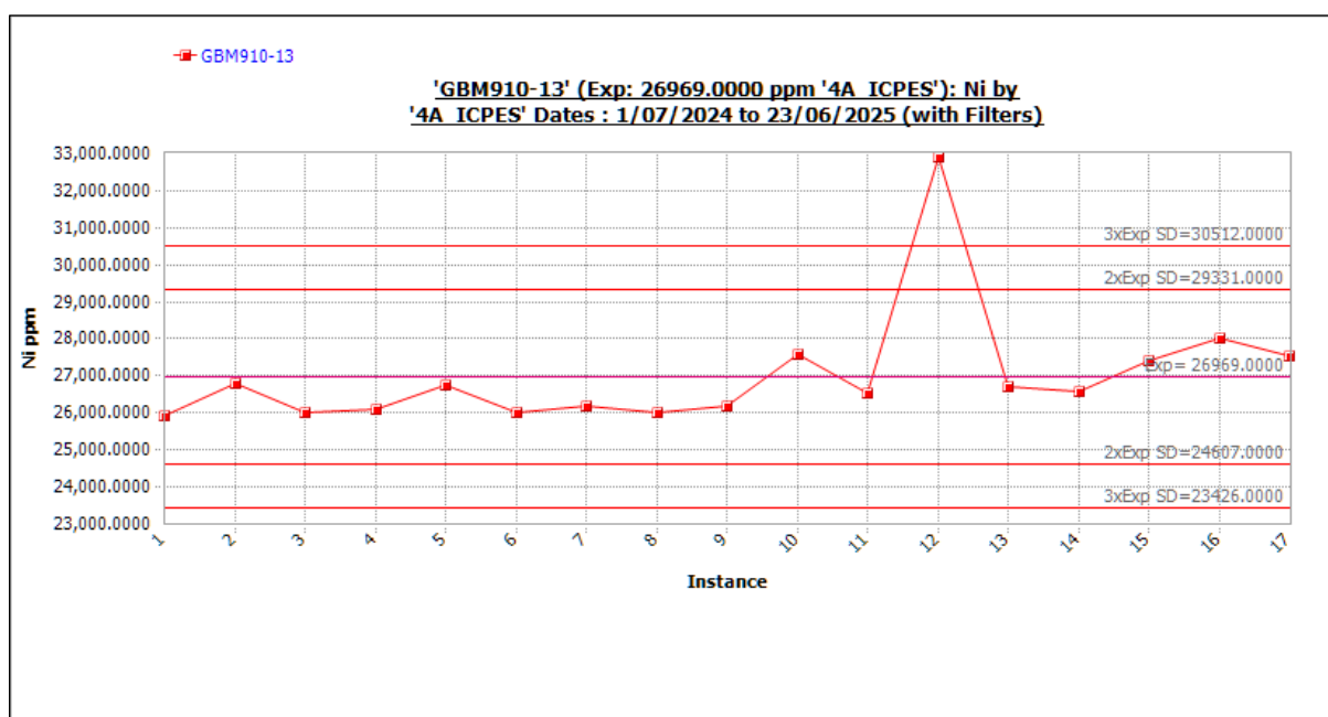
Figure 11-87 Standard GBM910-13 outliers included. Source: Westgold.
