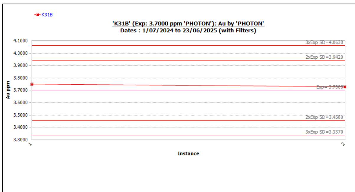
Figure 11-51 Standard K31B outliers included. Source: Westgold.
