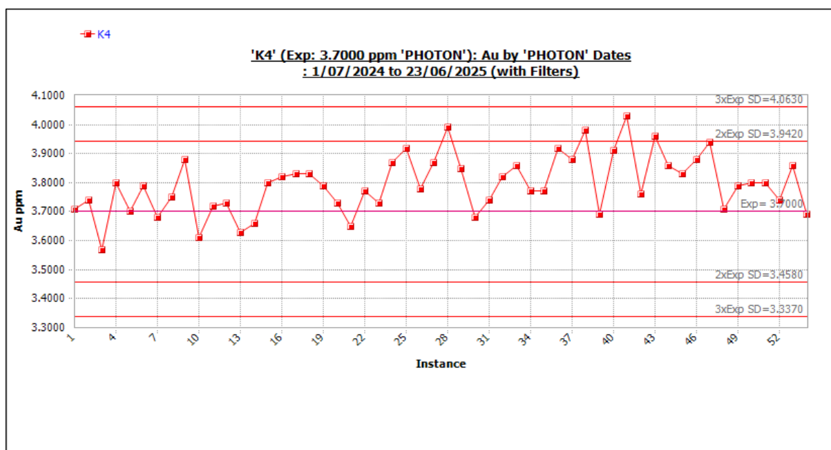
Figure 11-61 Standard K4 outliers included. Source: Westgold.
