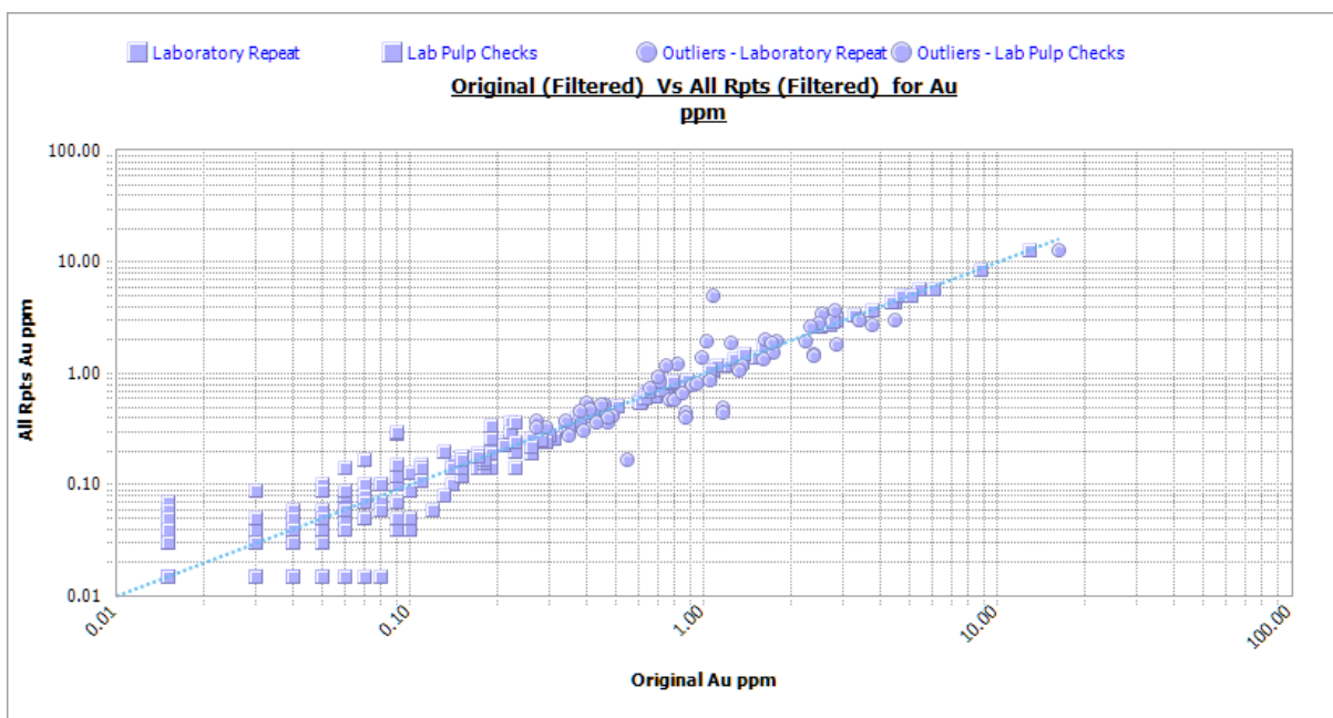
Figure 11-83 Scatter plot Photon Assay - drillhole (repeat code) : original vs all repeats for Au ppm. Source: Westgold.
