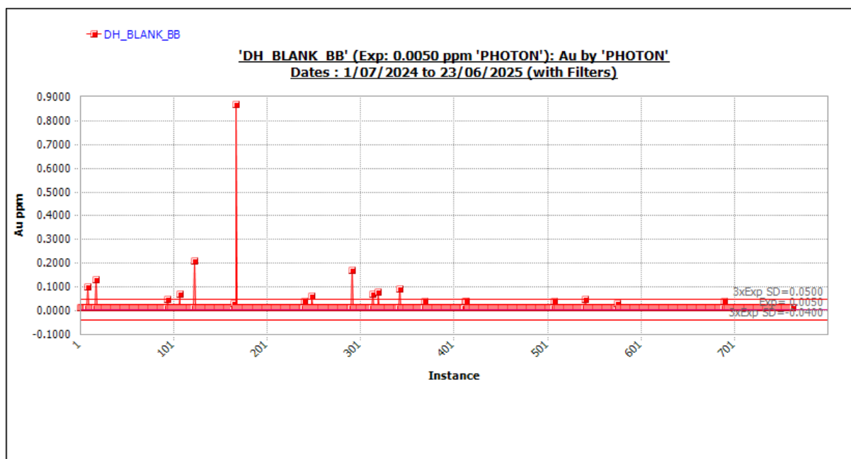
Figure 11-8 Standard DH_BLANK_BB outliers included. Source: Westgold.
