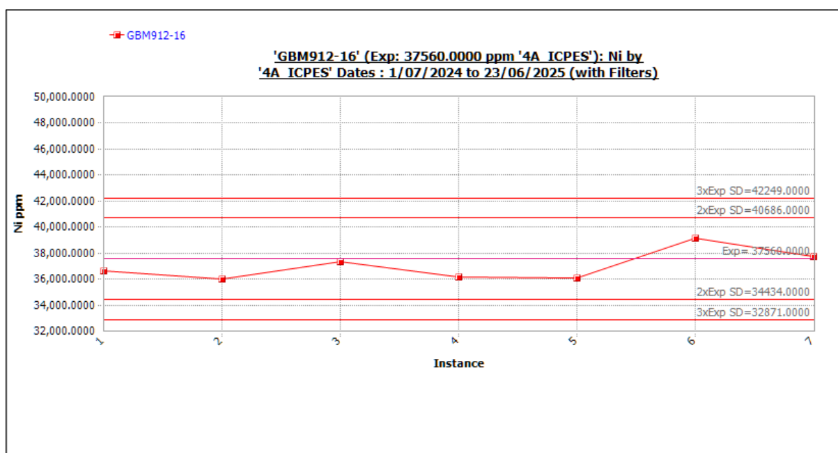
Figure 11-89 Standard GBM912-16 outliers included. Source: Westgold.
