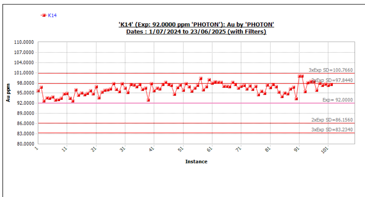
Figure 11-27 Standard K14 outliers included. Source: Westgold.
