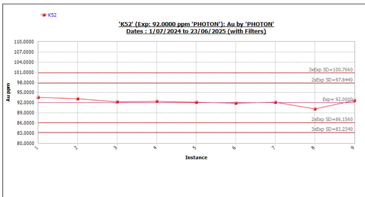
Figure 11-75 Standard K52 outliers included. Source: Westgold.
