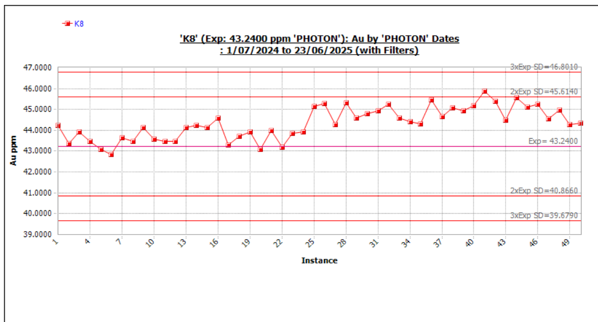
Figure 11-80 Standard K8 outliers included. Source: Westgold.
