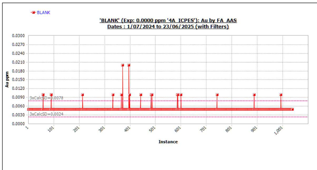
Figure 11-6 Standard BLANK outliers included. Source: Westgold.
