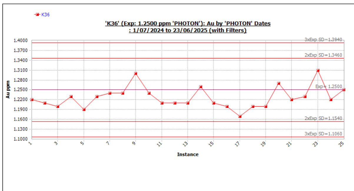
Figure 11-57 Standard K36 outliers included. Source: Westgold.
