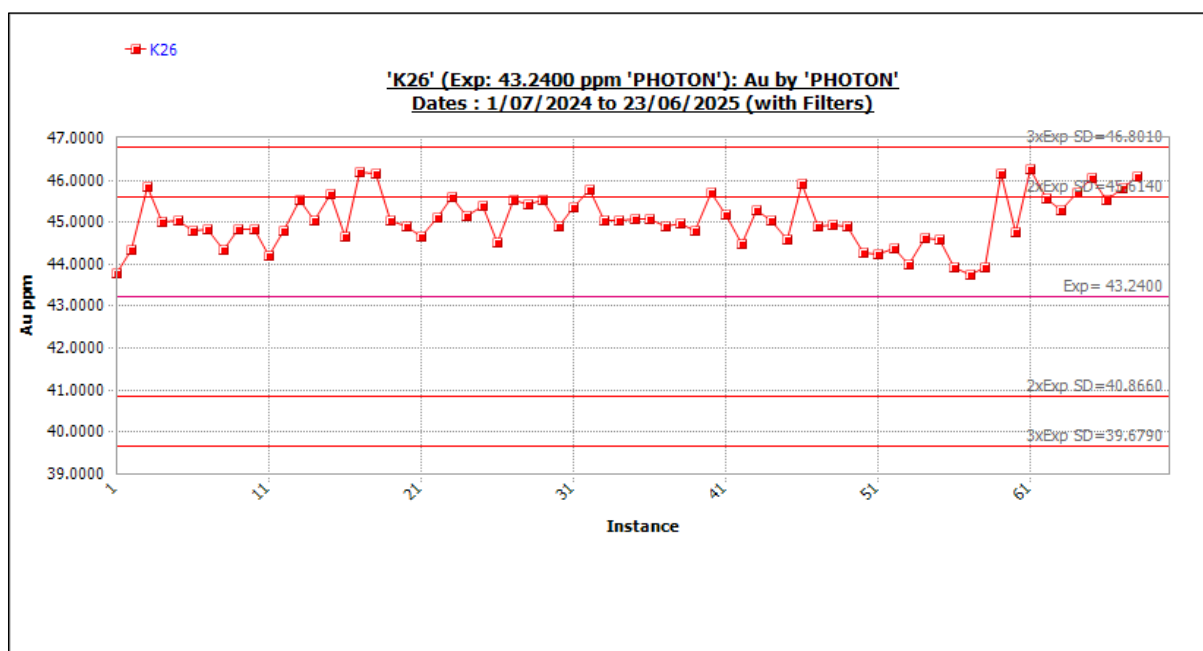
Figure 11-43 Standard K26 outliers included. Source: Westgold.
