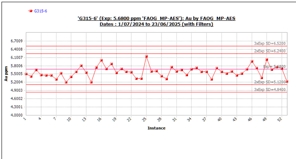
Figure 11-9 Standard G315-6 outliers included. Source: Westgold.
