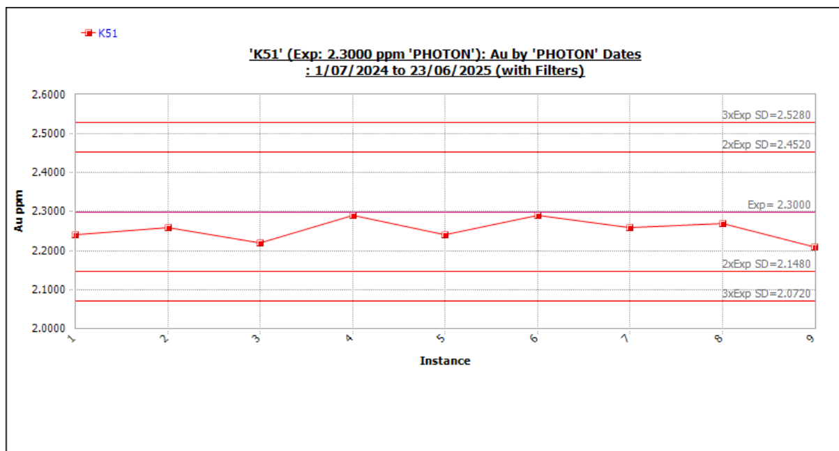
Figure 11-74 Standard K51 outliers included. Source: Westgold.
