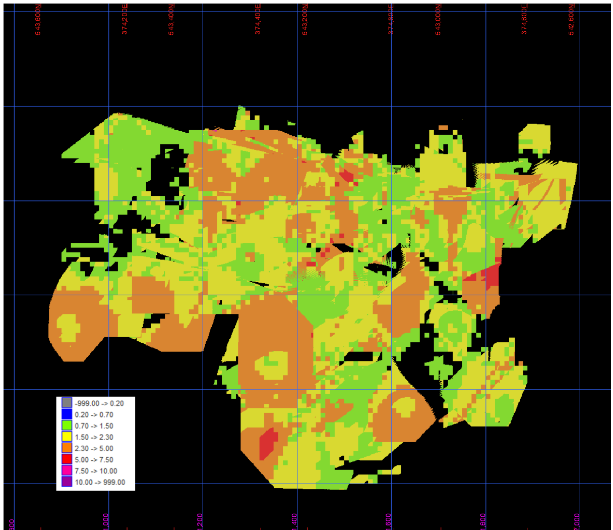
Figure 14-37 Fletcher depleted Mineral Resource Estimate, constrained to 1.2 g/t COG for Indicated and Inferred classified material only - Source : Westgold.
