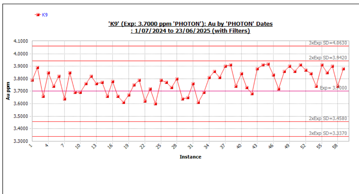
Figure 11-81 Standard K9 outliers included. Source: Westgold.
