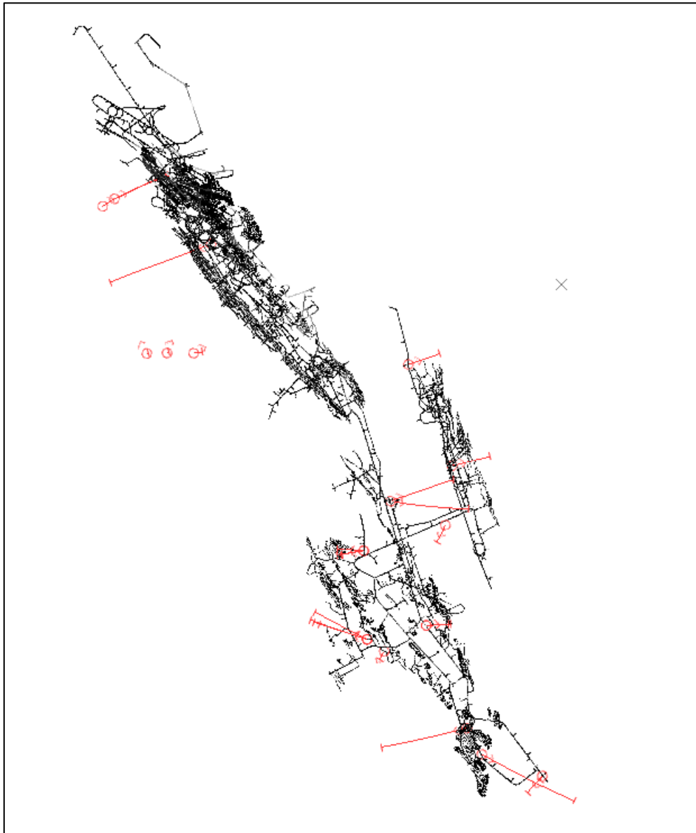
Figure 10-5 location of holes subject to gold resample work completed during the reporting period – Source : Westgold.
