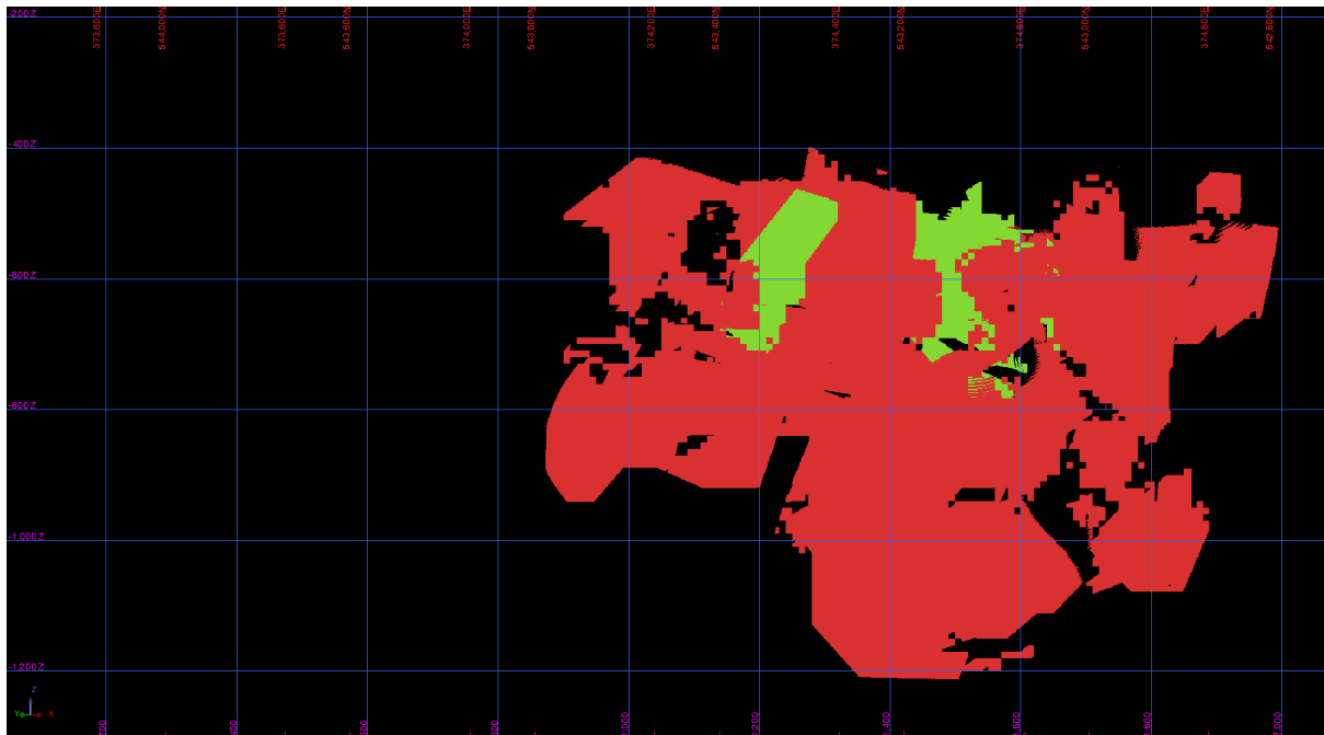
Figure 14-38 Fletcher Mineral Resource Classification for the reported resource. Green = Indicated, red = Inferred - Source : Westgold.
