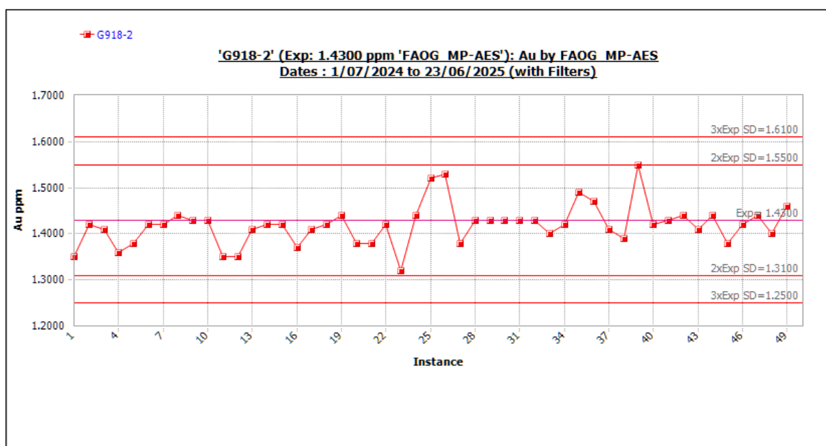
Figure 11-21 Standard G918-2 outliers included. Source: Westgold.
