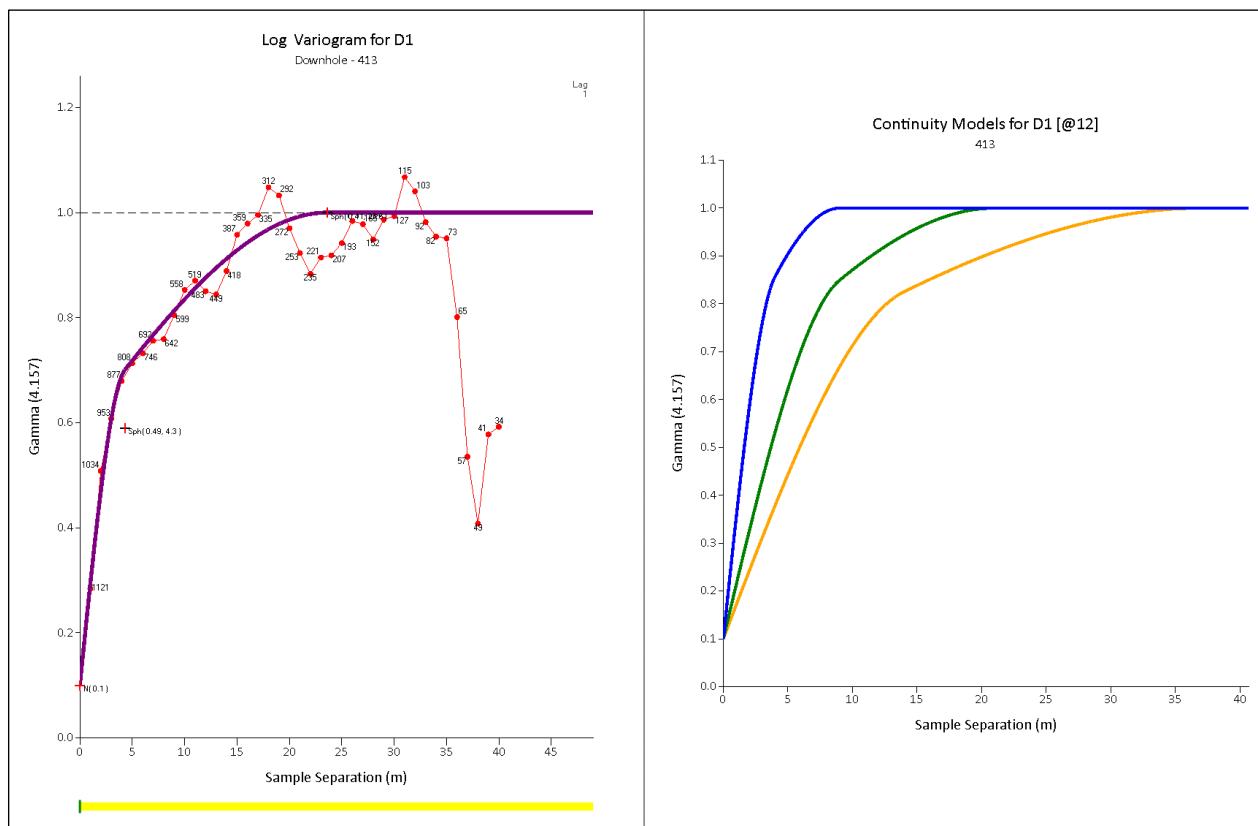
Figure 14-23 Larkin downhole variogram and continuity models – Domain 413– Source : Westgold.
