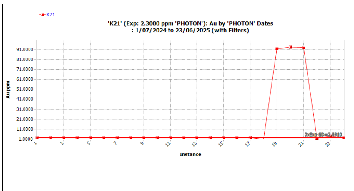
Figure 11-33 Standard K21 outliers included. Source: Westgold.
