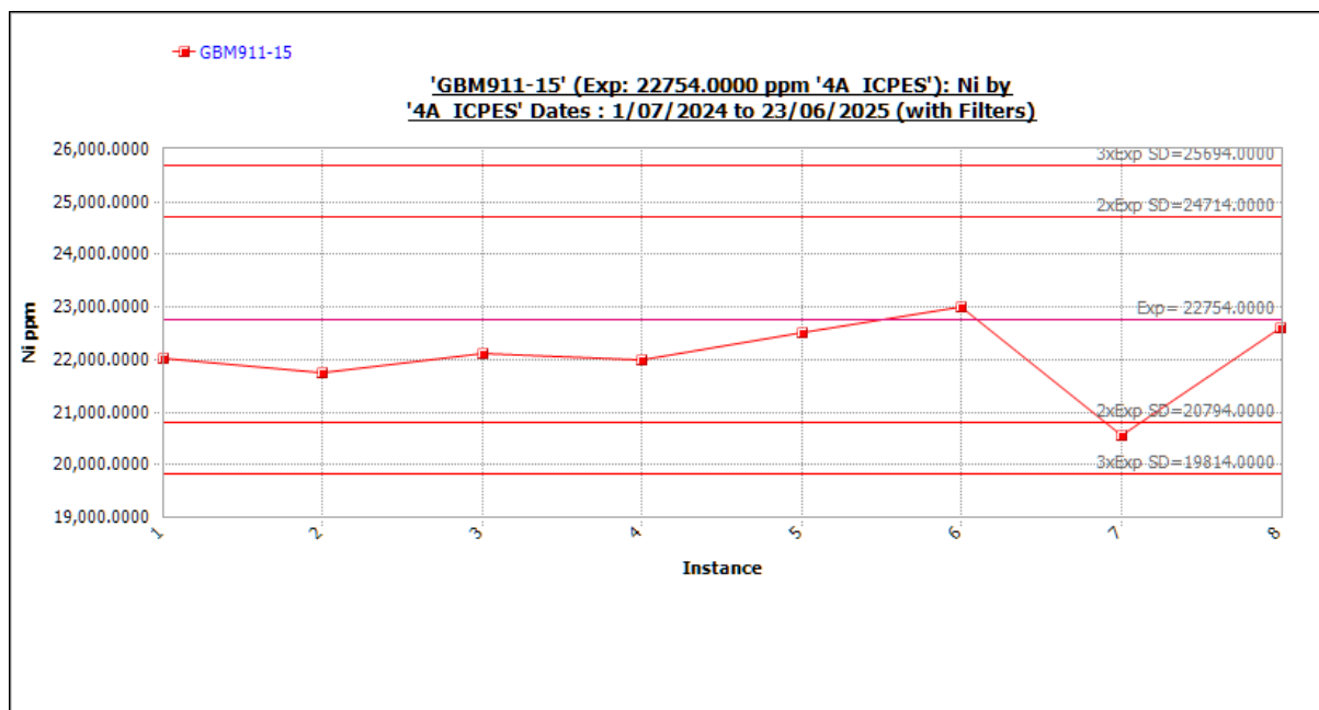
Figure 11-86 Standard GBM911-15 outliers included. Source: Westgold.
