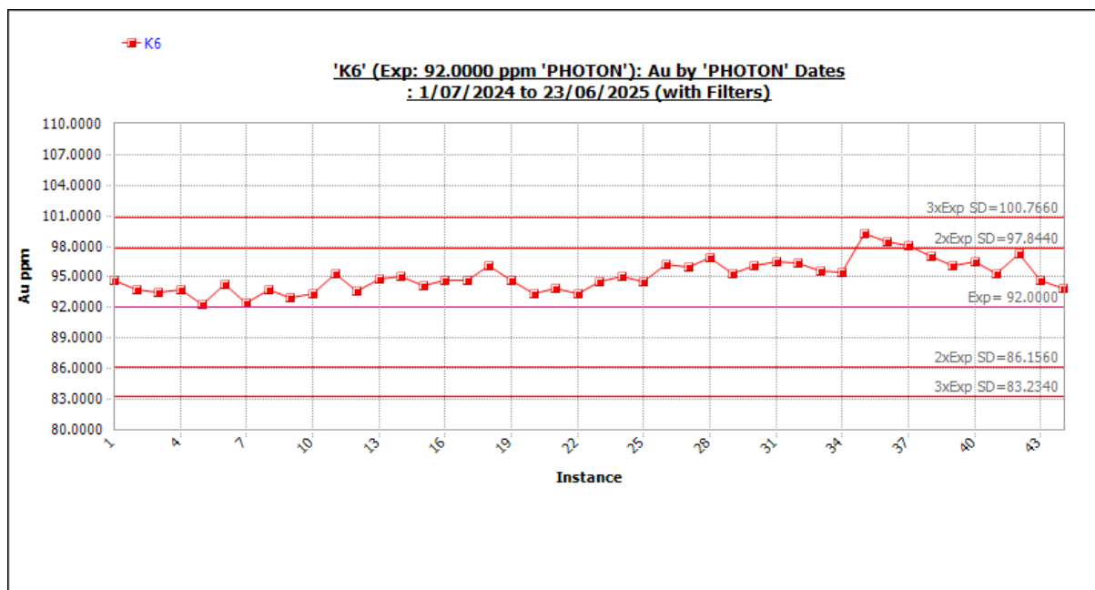
Figure 11-78 Standard K6 outliers included. Source: Westgold.
