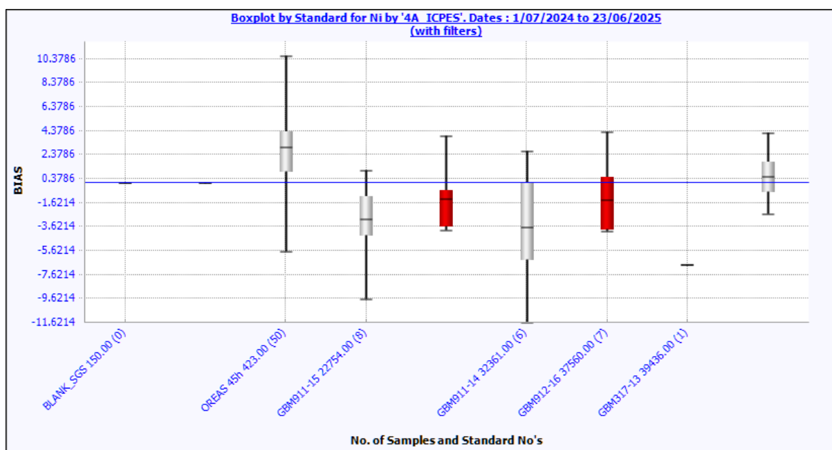
Figure 11-84 Standards – sRPD box and whisker plot SGS Perth four acid digest ICPES. Source: Westgold.
