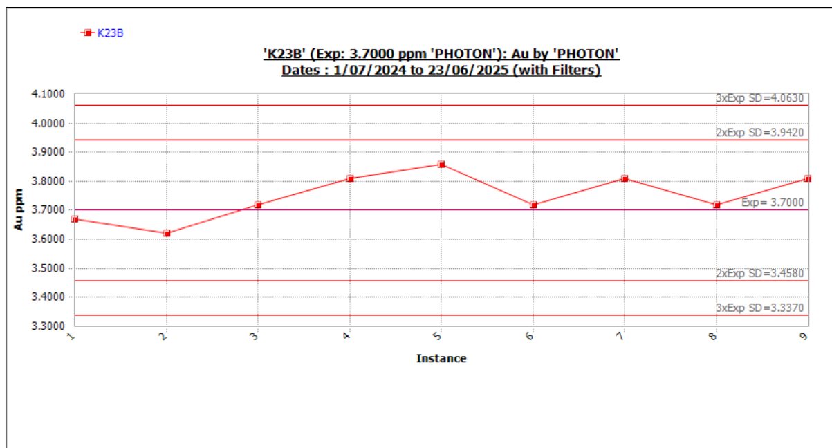
Figure 11-38 Standard K23B outliers included. Source: Westgold.
