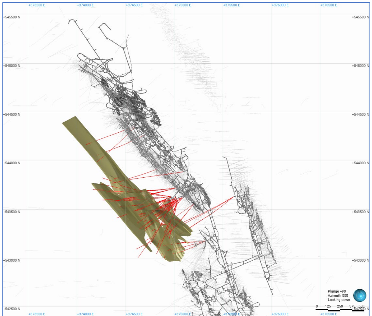
Figure 14-34 Plan view of Fletcher deposit, drillholes intersecting mineralisation domains in red - Source : Westgold.
