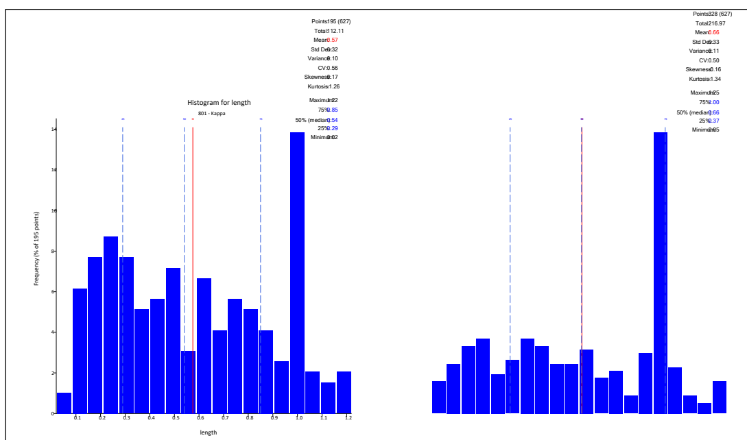
Figure 14-44 Raw sample length statistics for Kappa and Delta – Source : Westgold.
