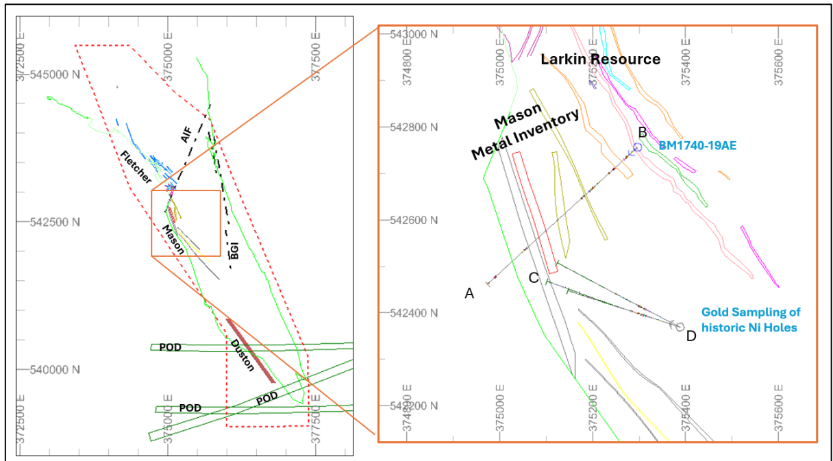
Figure 10-3 Plan View showing the new drill hole to test the western extension, and the historic resample holes testing the southern extension of Mason – Source : Westgold.
