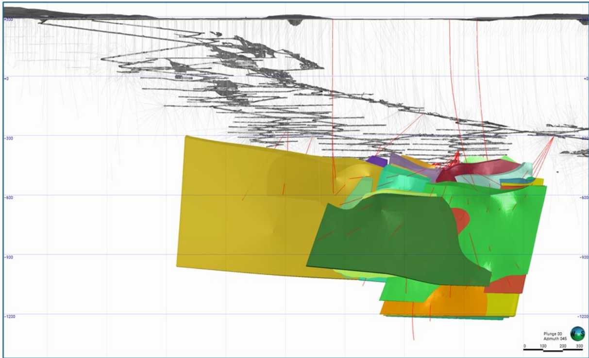
Figure 14-35 Fletcher mineralisation domains – oblique view looking northeast (local KNO grid) - Source : Westgold.
