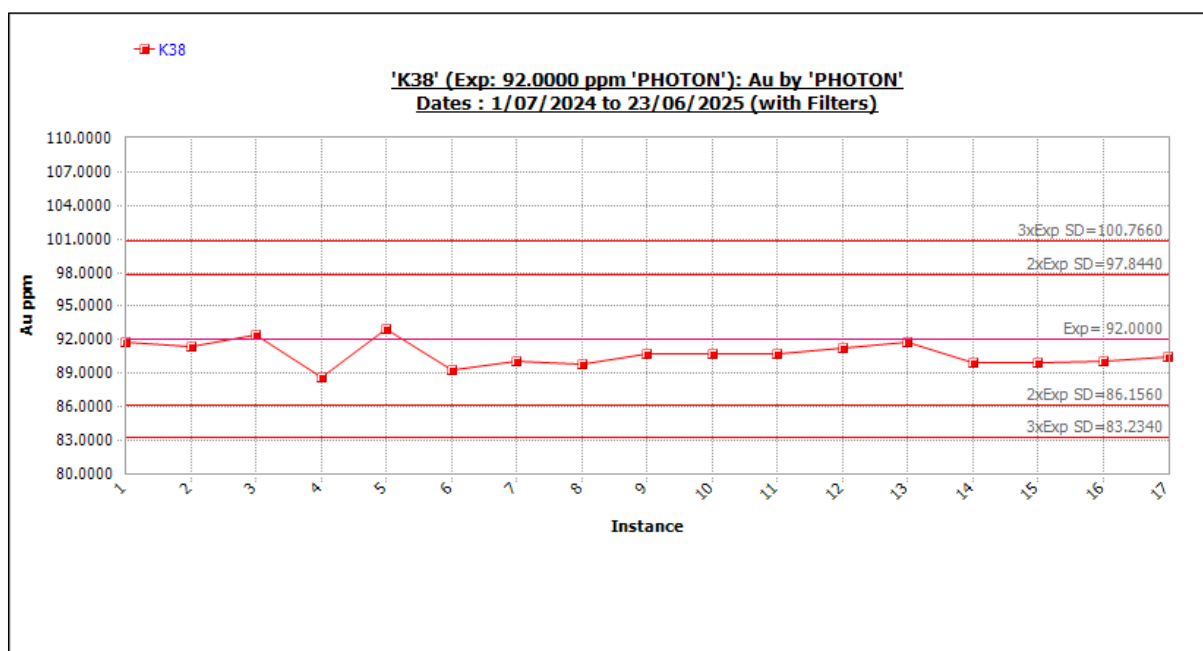
Figure 11-59 Standard K38 outliers included. Source: Westgold.
