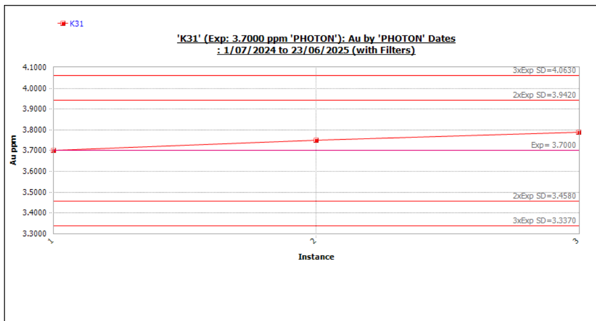
Figure 11-50 Standard K31 outliers included. Source: Westgold.
