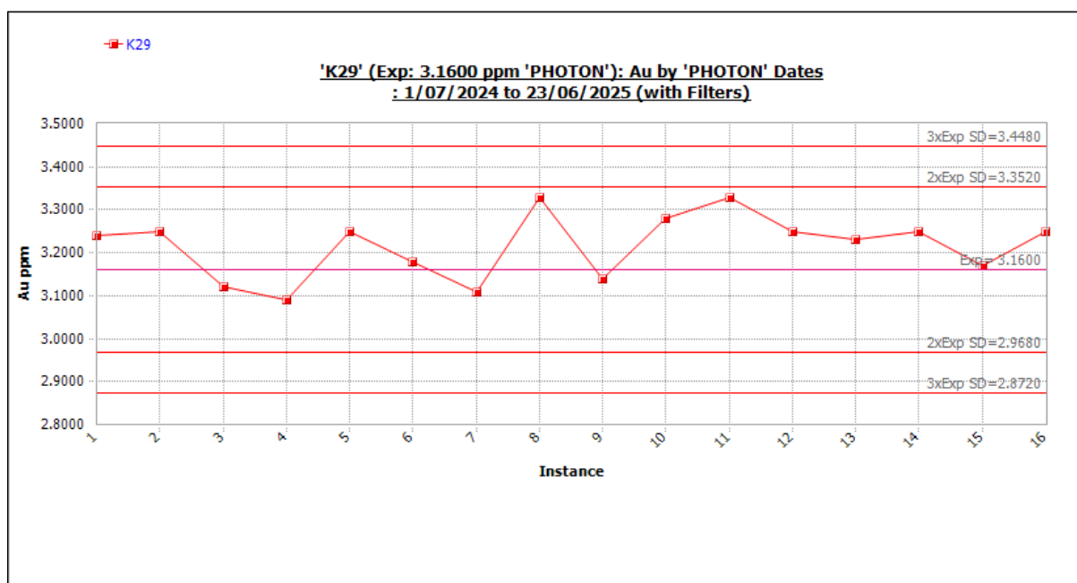
Figure 11-47 Standard K29 outliers included. Source: Westgold.
