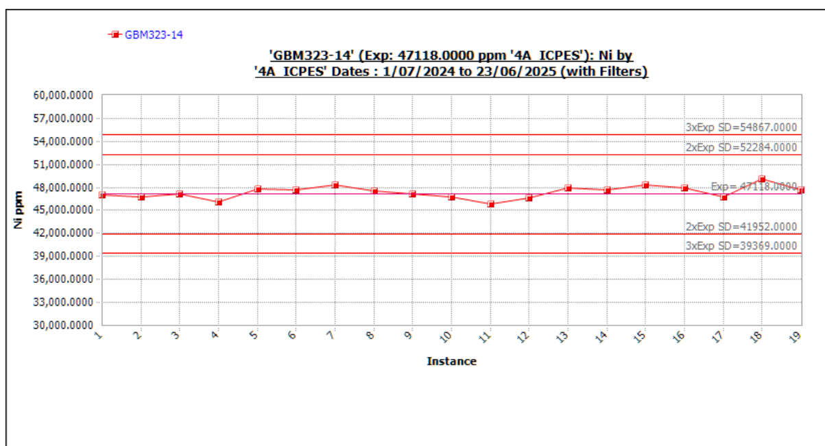
Figure 11-90 Standard GBM323-14 outliers included. Source: Westgold.
