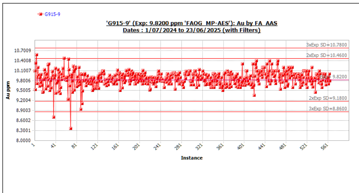
Figure 11-18 Standard G915-9 outliers included. Source: Westgold.
