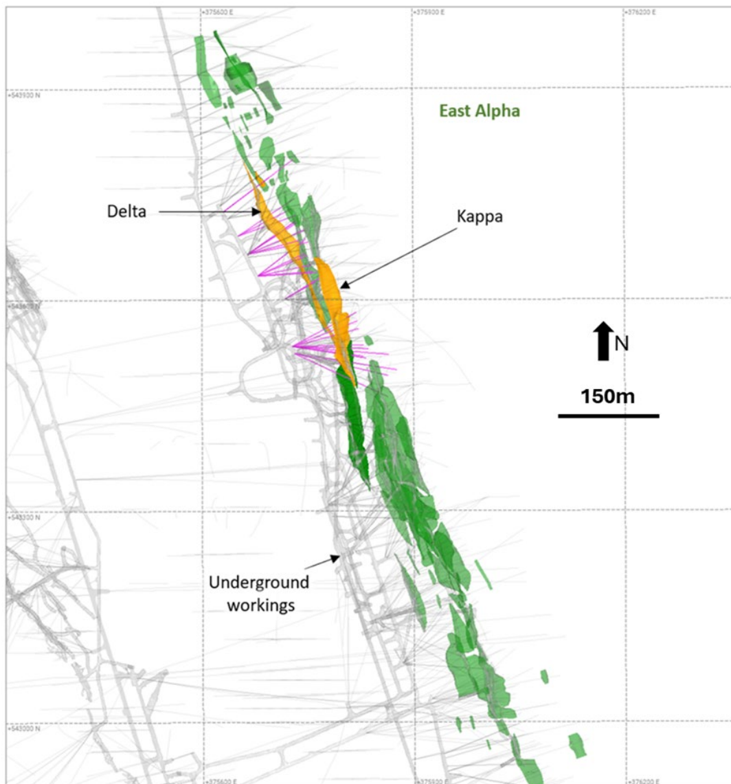
Figure 14-42 Location plan of Kappa and Delta lenses at East Alpha showing new drilling in magenta – Source : Westgold.
