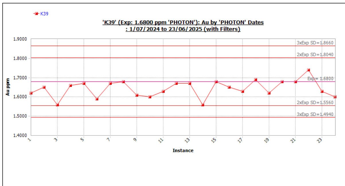
Figure 11-60 Standard K39 outliers included. Source: Westgold.
