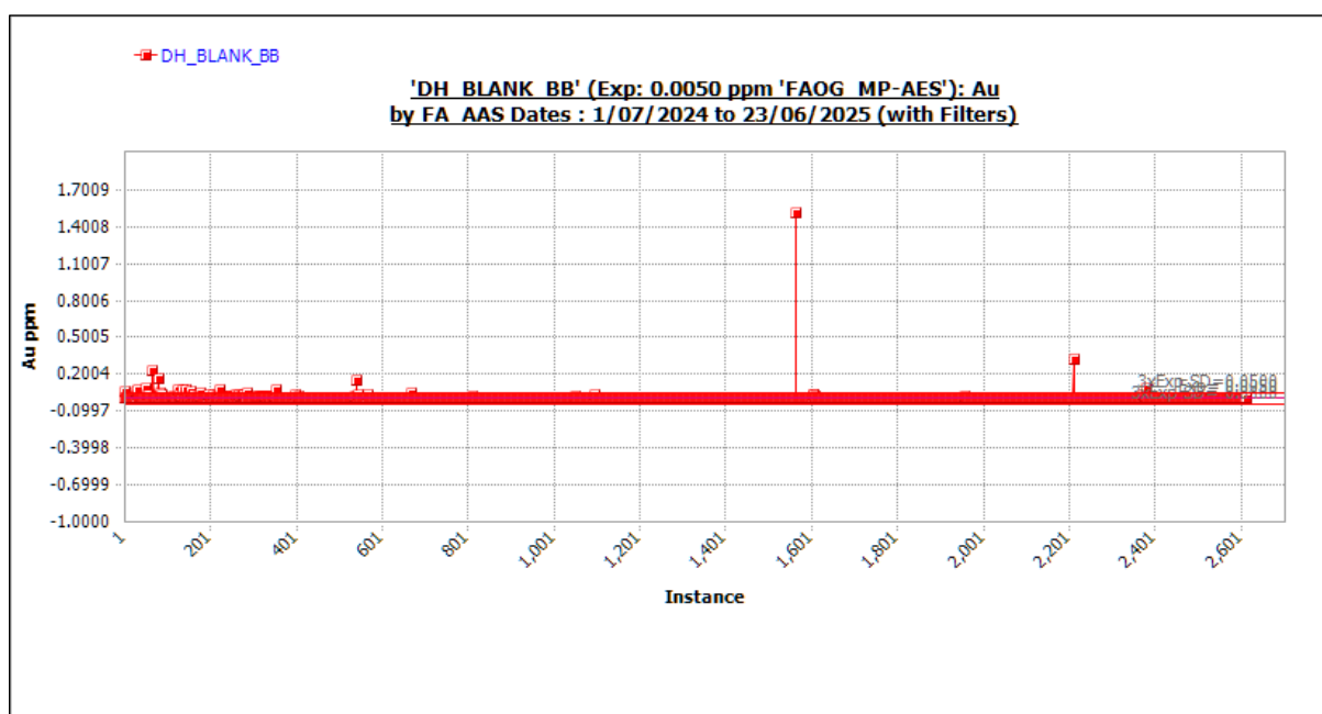
Figure 11-7 Standard DH_BLANK_BB outliers included. Source: Westgold.
