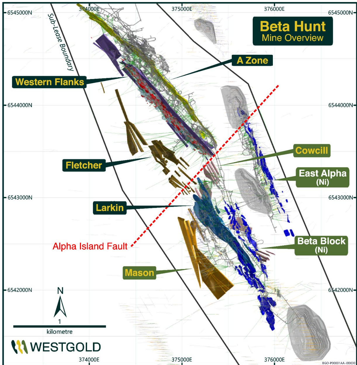
Figure 14-1 Beta Hunt Gold Deposit Location Plan – Source : Westgold.
