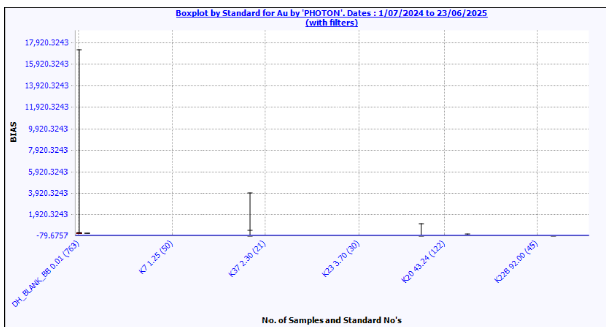
Figure 11-5 Standards - sRPD box and whisker plot SGS Perth PhotonAssay™. Source: Westgold.
