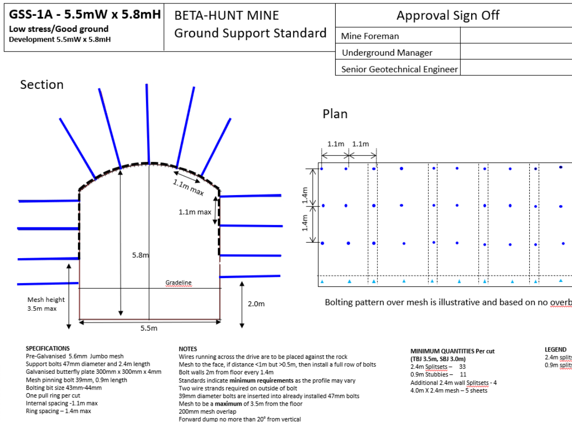
Figure 16-3 Typical ground support design – Source : Westgold.
