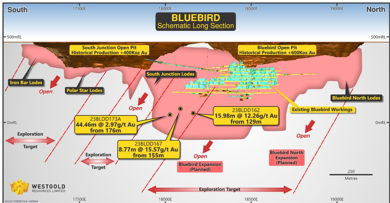
Figure 8: Bluebird schematic long-section showing significant intersections.
