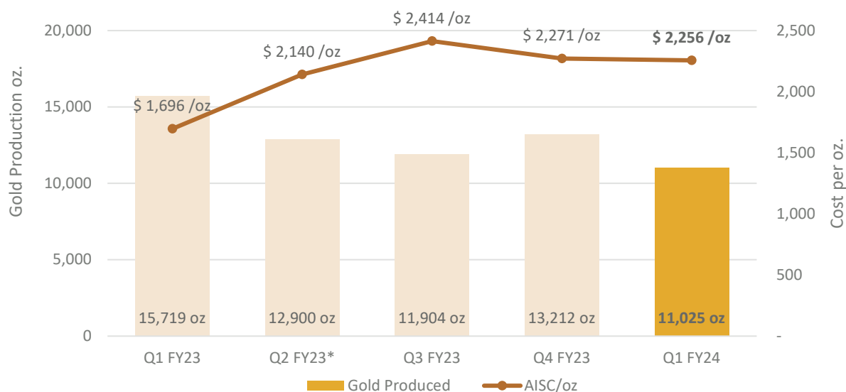
Figure 12: Bryah Gold Production and AISC
