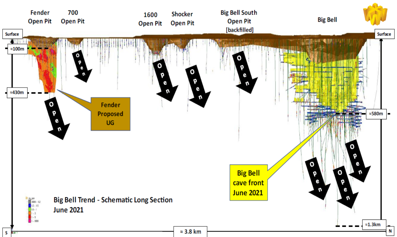
Figure 2 – Big Bell Trend Schematic Long-Section.
