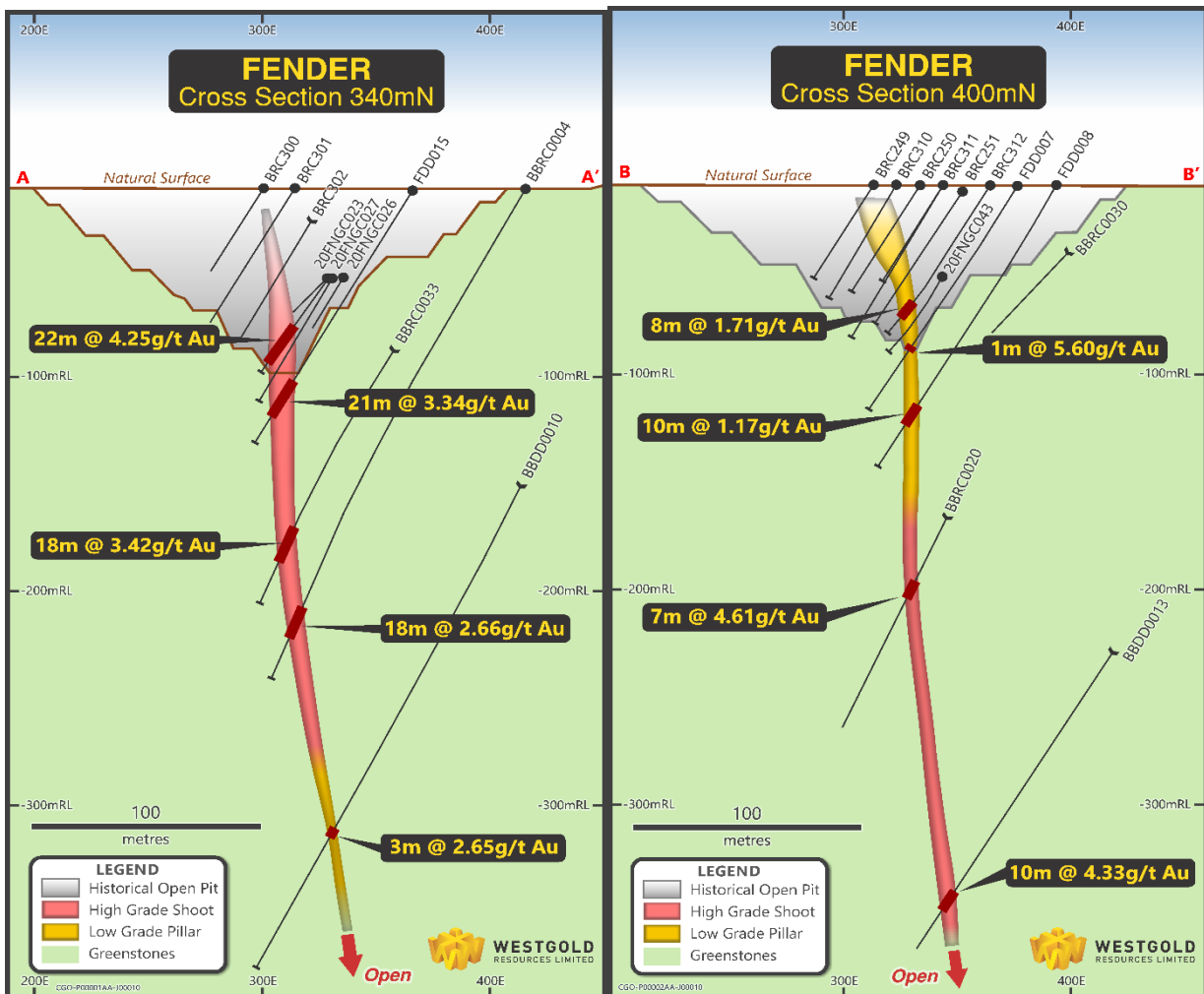
Figure 5 & 6 – Fender Cross-Sections at 340mN and 400mN [ looking north]
