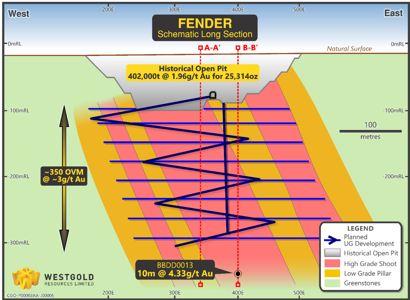
Figure 4 – Fender Schematic Long Section [with cross-sections A-A’ and B-B’ annotated]
