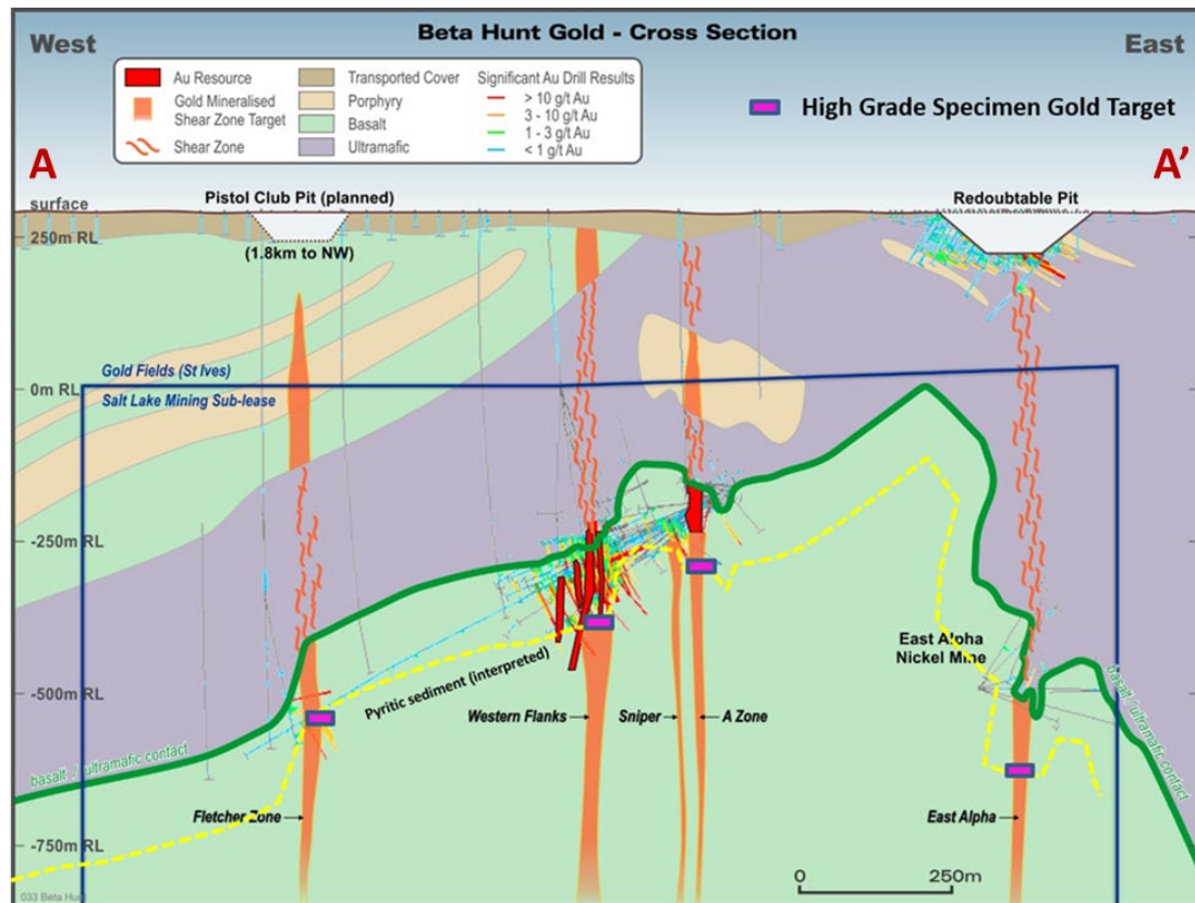
Figure 7-6 Composite cross-section looking north showing interpreted shear zone related gold mineralisation and rock type Source : Westgold.
