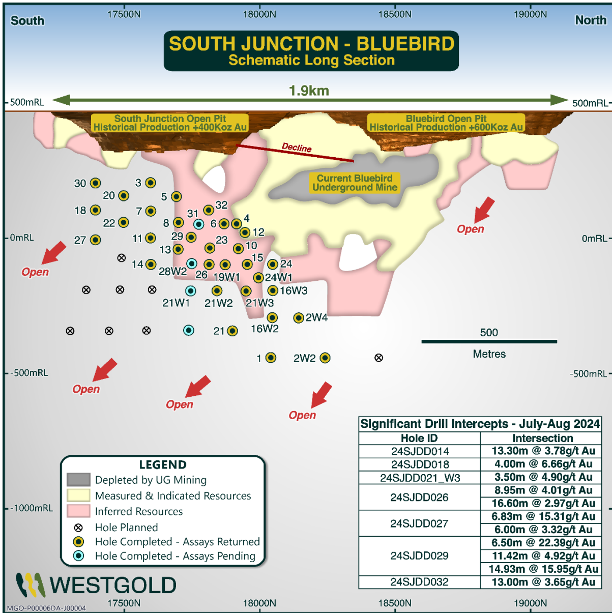
Figure 3 – Bluebird South Junction Long Section showing 2024 Resource Definition drill holes & significant intersections returned during July & August 2024 (for results of previously drilled holes refer to ASX Releases of 14 May and 2 July 2024).
