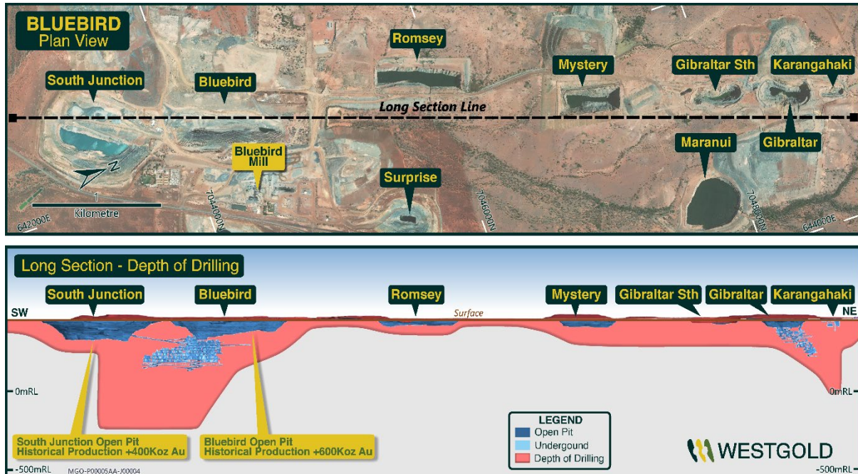
Figure 1 – Westgold Meekatharra operations showing historic open pits and the location of the Bluebird – South Junction mining complex.
