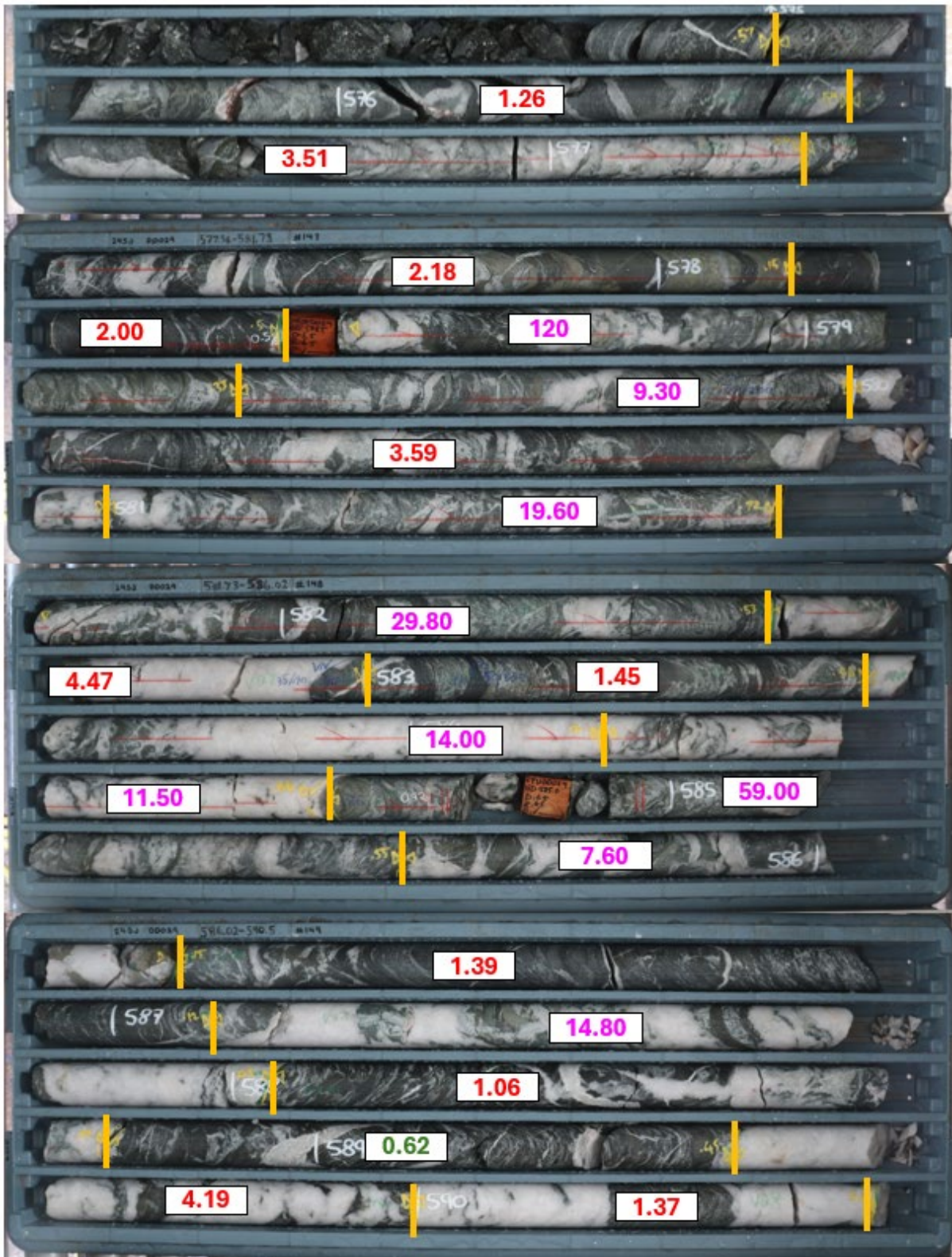
Figure 4 – South Junction Drill Hole 24SJDD029 showing the individual gold assay results (g/m) for the “South Junction Lode” (highly altered and quartz veined ultramafics) which returned 14.93m @ 15.95g/t Au from 575.57m (Refer to Appendix A for details).
