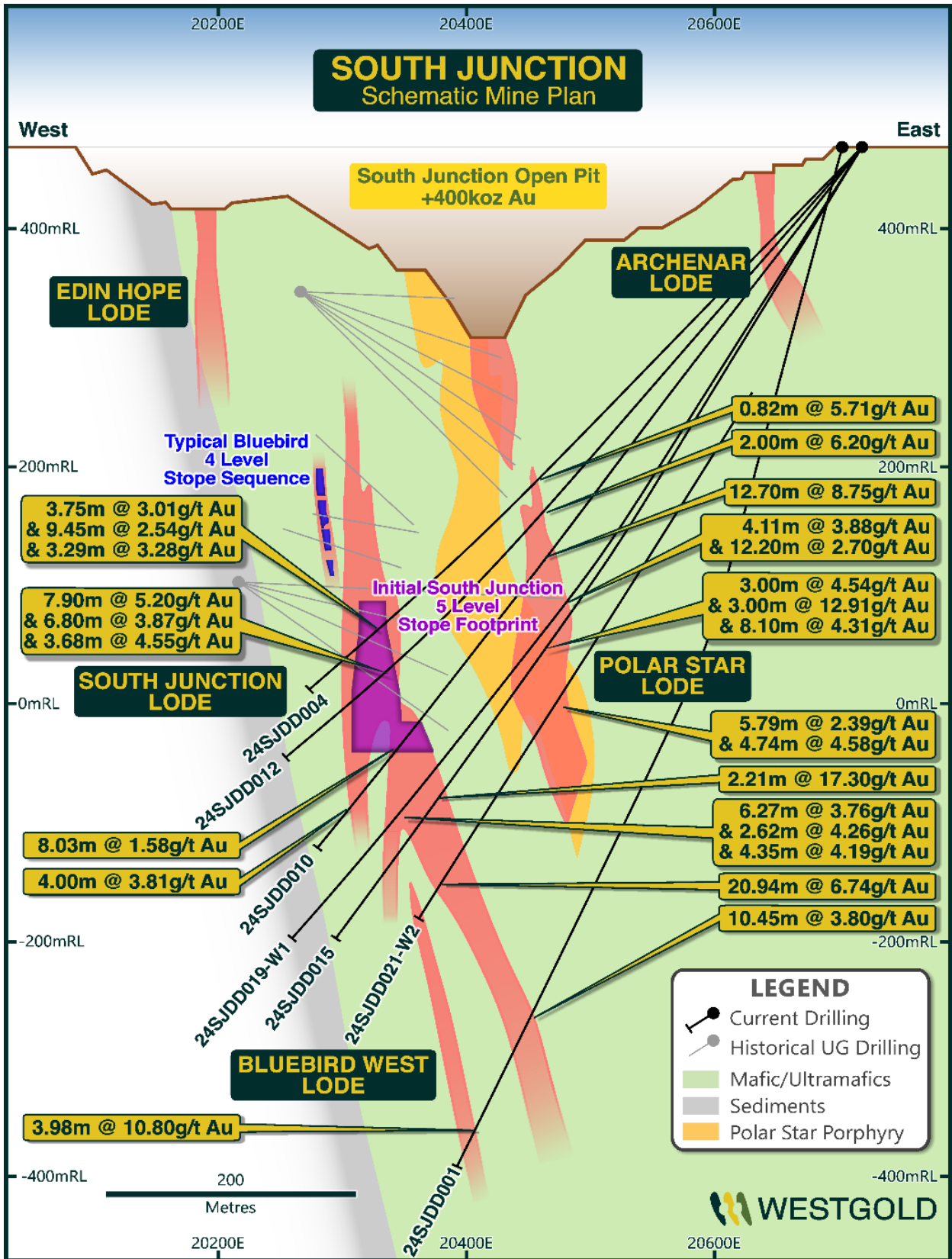
Figure 2 -- Schematic cross section showing location of the recently commenced mining on the South Junction Lode and the relative position of the Polar Star Lode (Refer ASX & TSX release of 14 August 2024 - "Westgold Declares Maiden South Junction Ore Reserve" for full drilling details)
